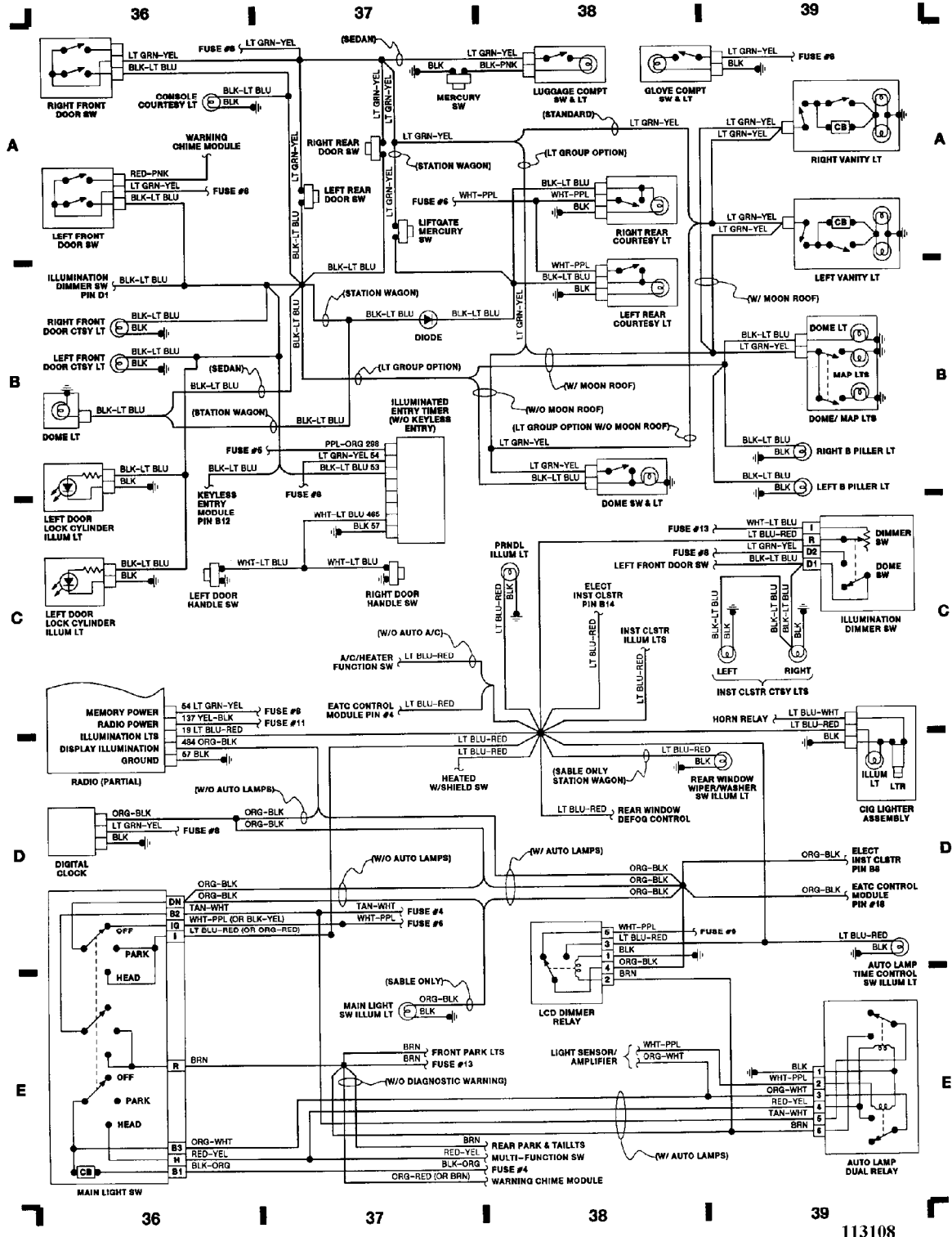
Fig. 10: Accessories
