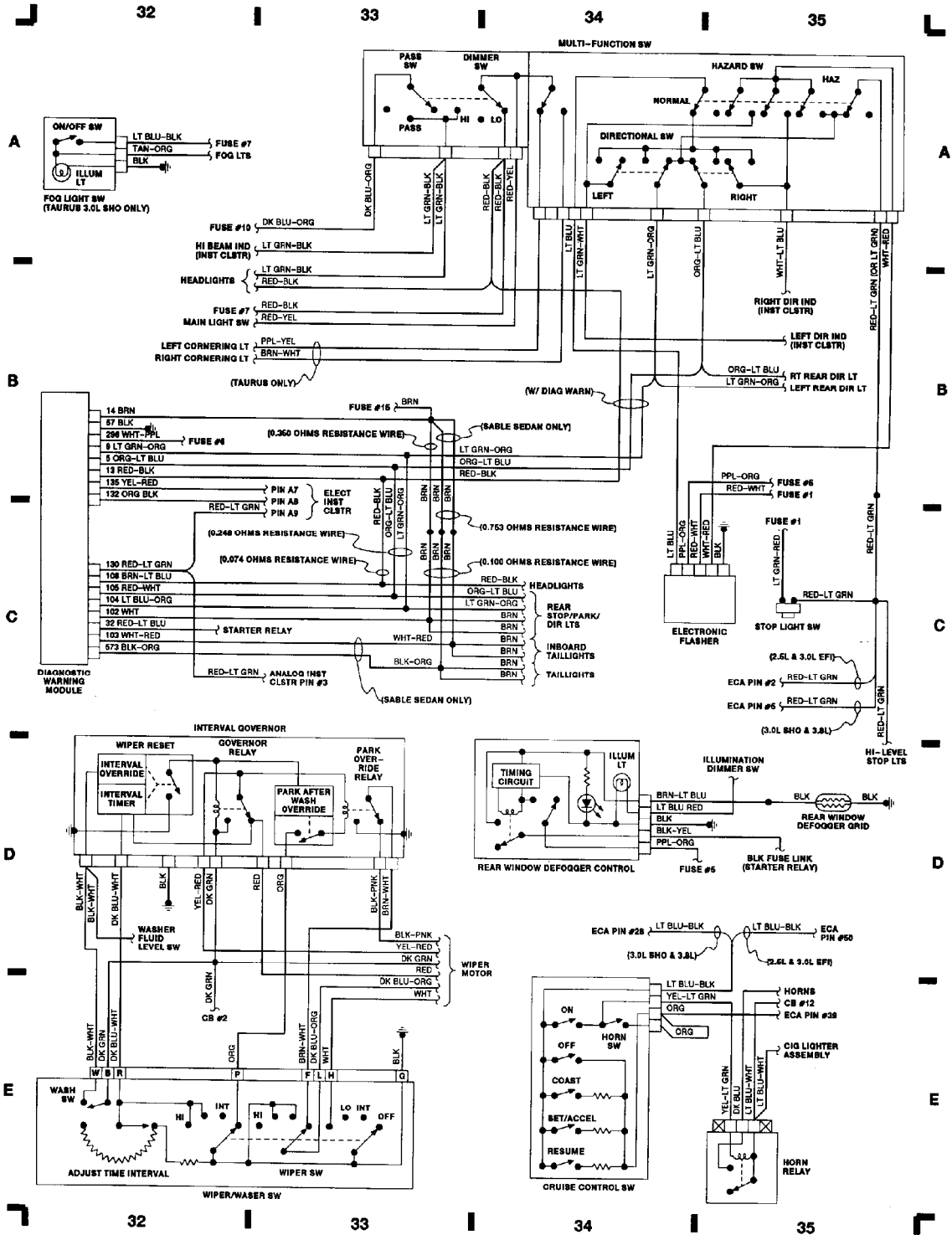
Fig. 9: Multi-Function Switch, Wiper/Washer System & Diagnostic Module
