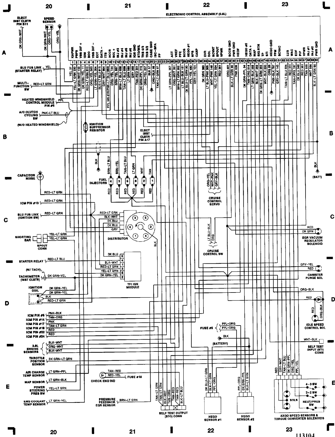
Fig. 6: Computer Engine Control (3.8L)
