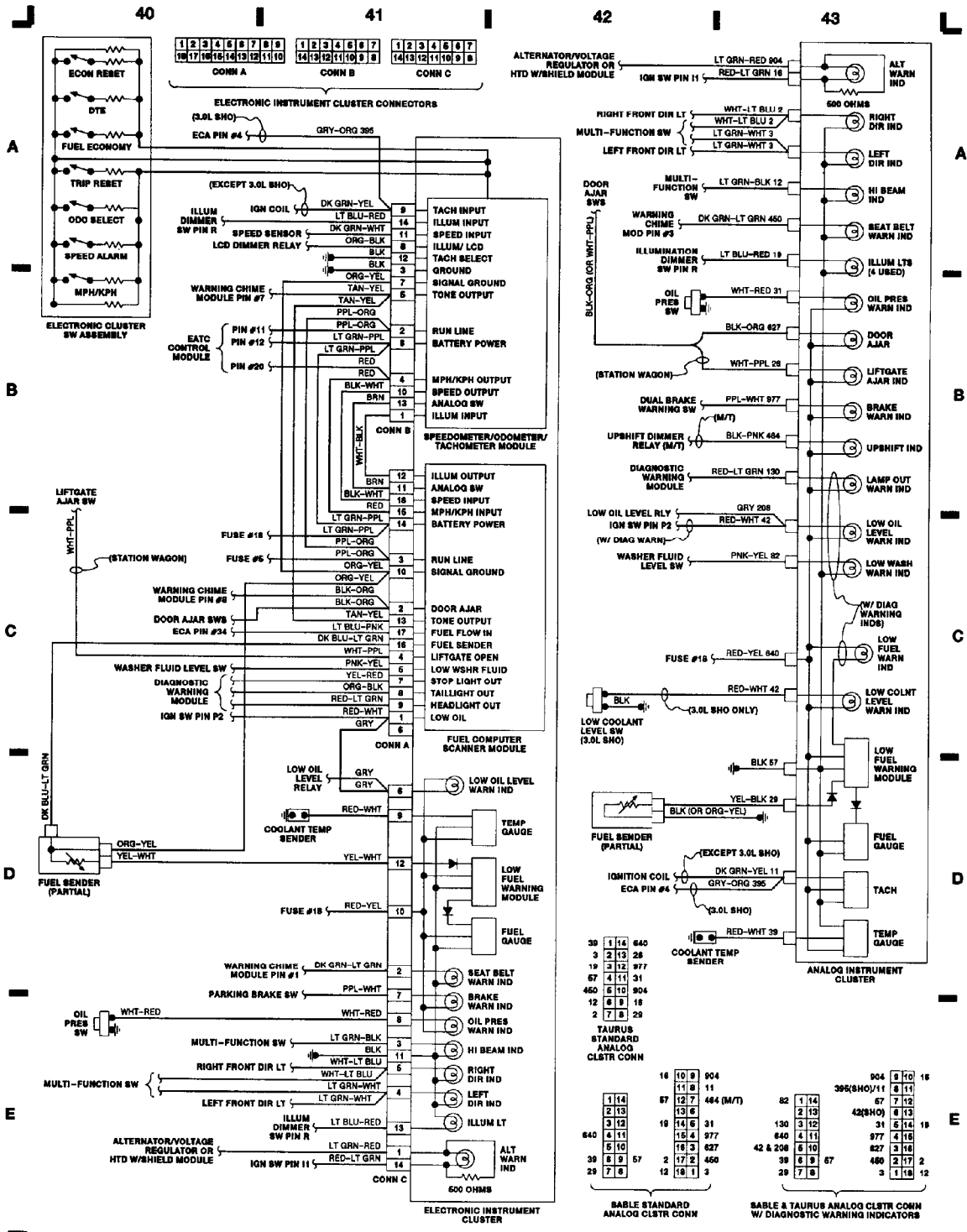
Fig. 11: Instrument Panel
