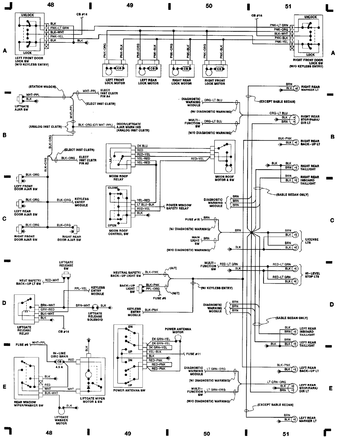
Fig. 13: Passenger Compartment (Cont.) & Taillights
