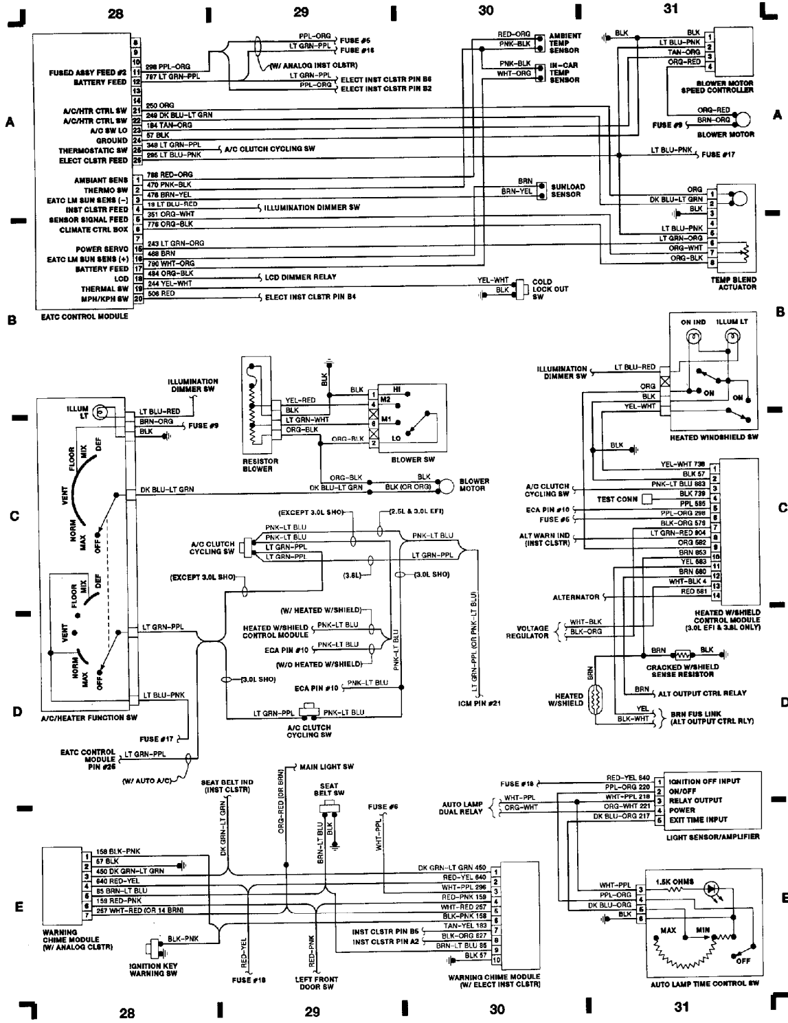
Fig. 8: A/C & Heater
