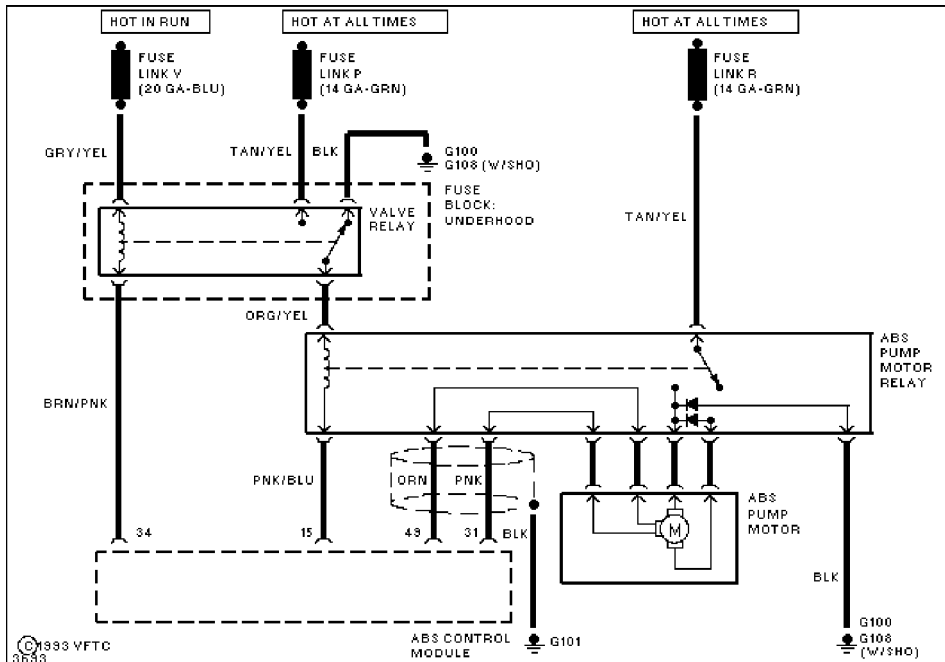
Fig. 14: Anti-Lock Brakes - Pump Circuit
