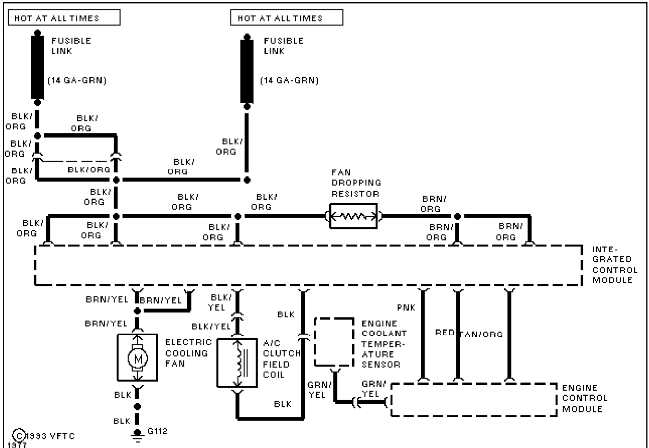
Fig. 18: Cooling Fan Circuit (3.0L Except SHO)
