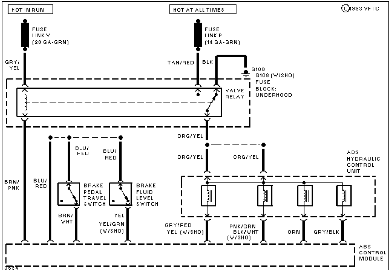
Fig. 15: Anti-Lock Brakes - Rear Valve Circuit
