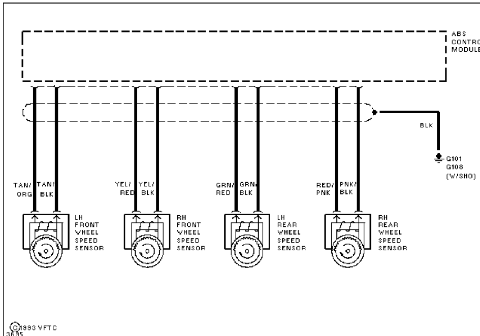
Fig. 16: Anti-Lock Brakes - Wheel Speed Sensor Circuit
