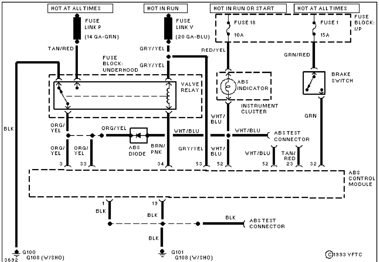
Fig. 13: Anti-Lock Brakes - Power Circuit
