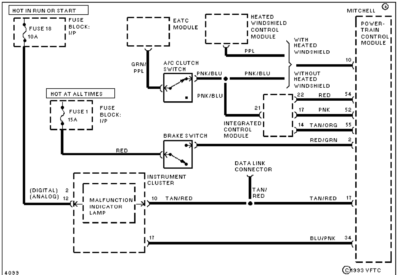
Fig. 35: Warning Indicator & A/C Control (3.0L)
