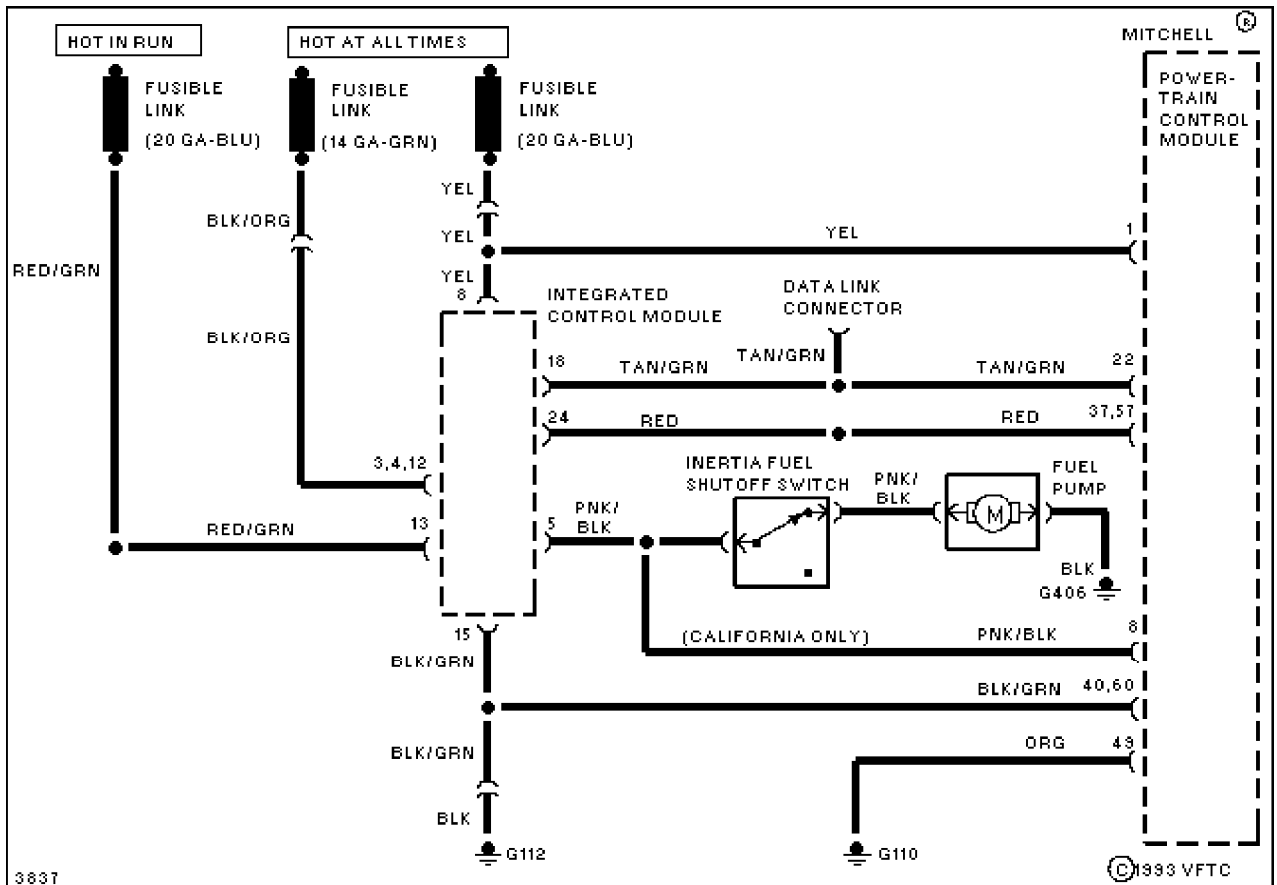
Fig. 33: Power, Ground & Fuel Pump Circuit (3.0L)
