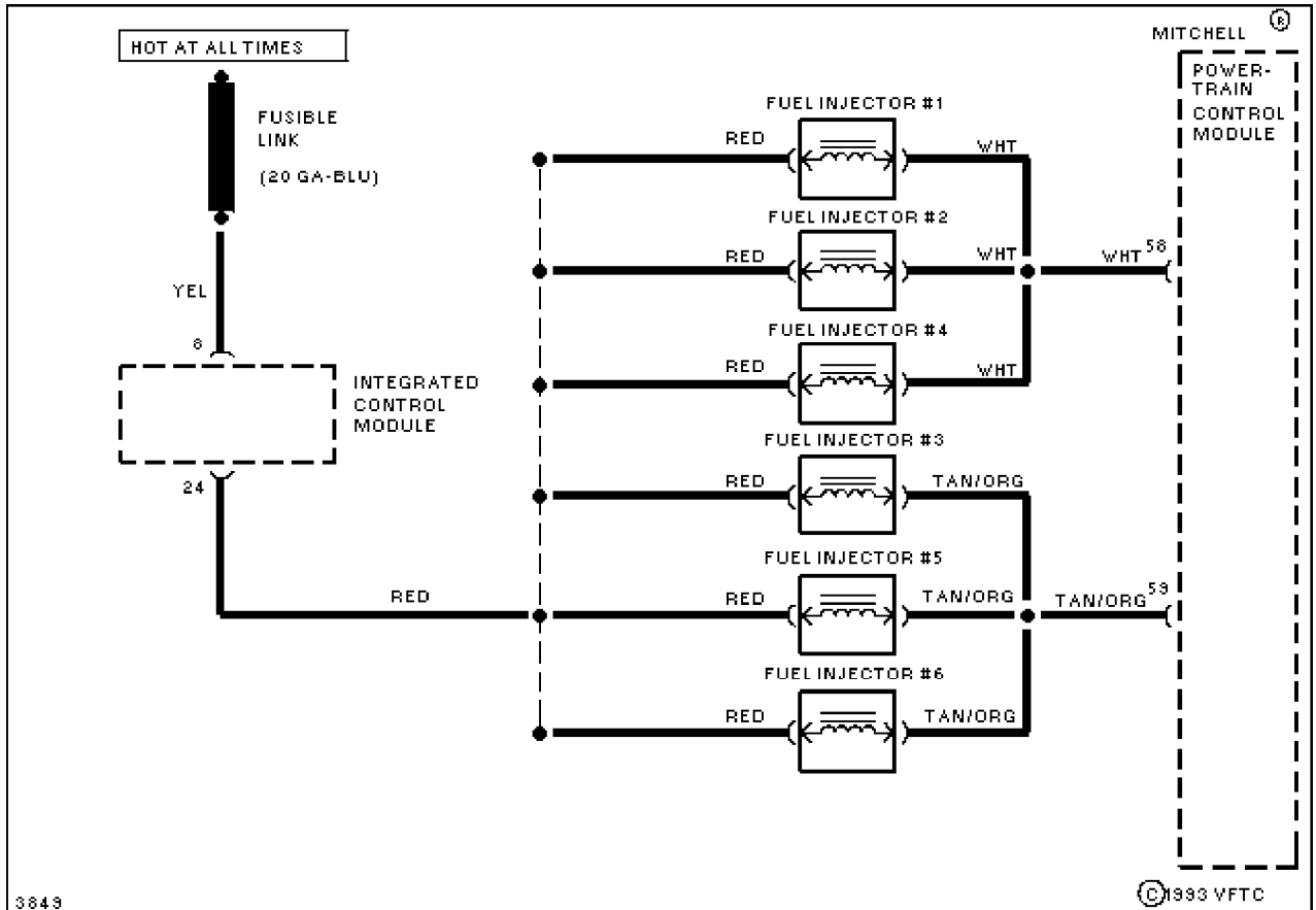
Fig. 31: Fuel Injector Circuit (3.0L)
