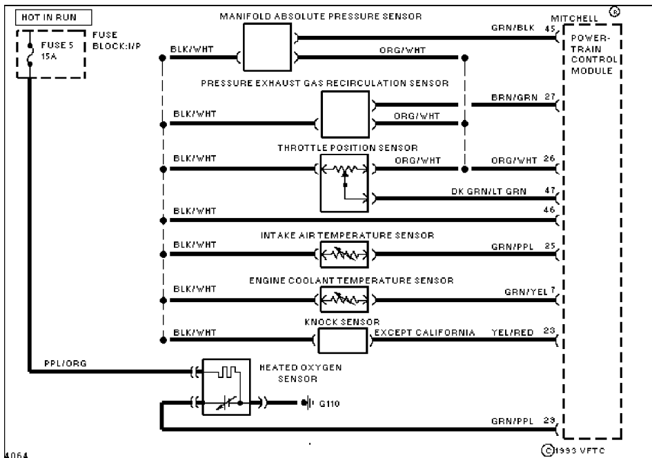
Fig. 34: Sensor & Valve Control Circuit (3.0L)
