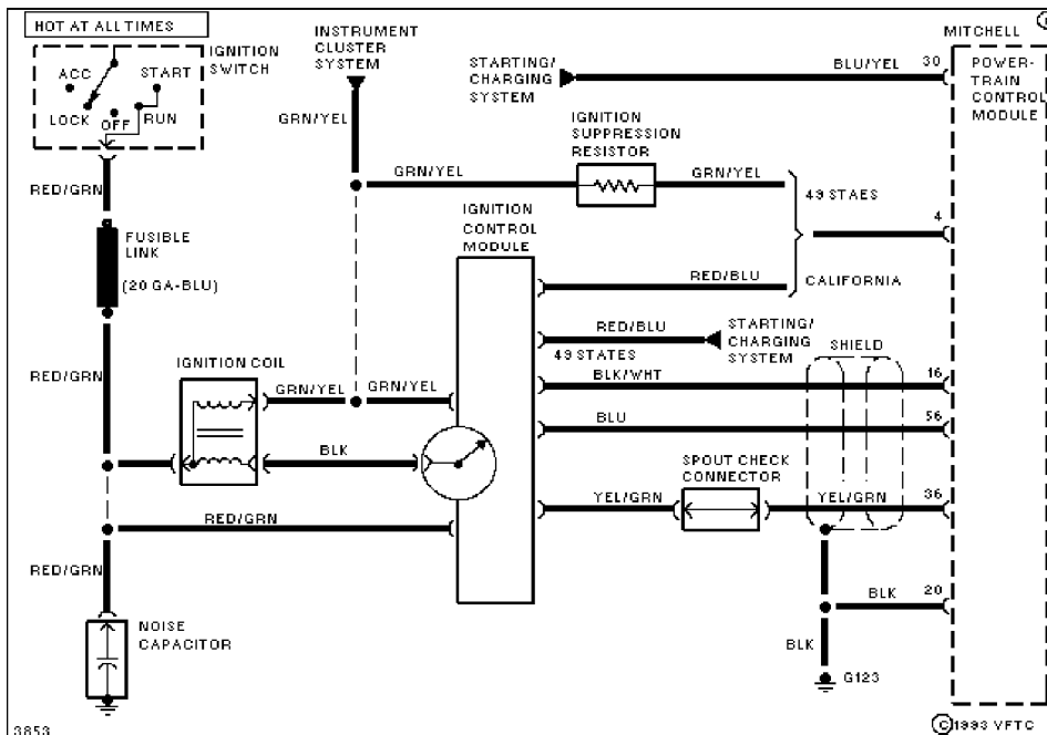
Fig. 32: Ignition Circuit (3.0L)
