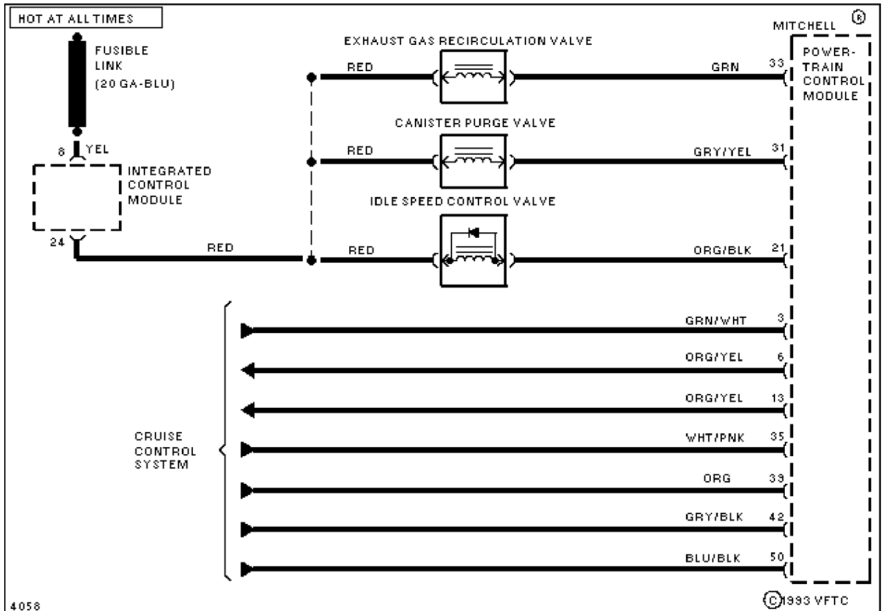
Fig. 30: Cruise & Valve Control Circuit (3.0L)
