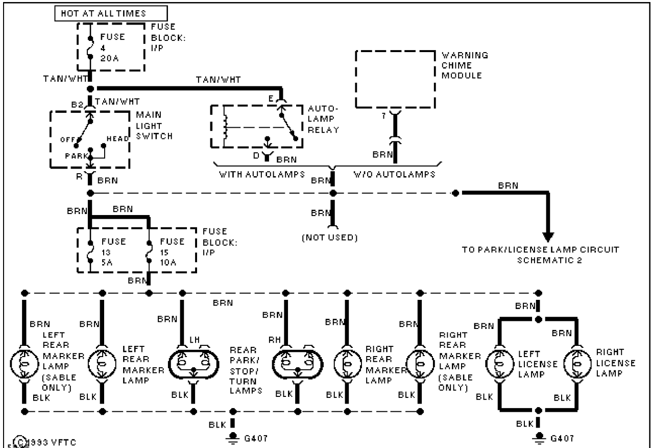
Fig. 48: Park/License Lamps (Sedan W/O Lamp Out Warning) (1 of 2)
