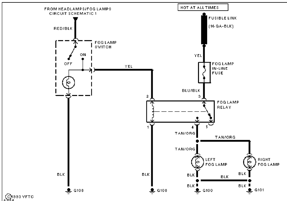
Fig. 56: Headlamps/Fog Lamps (2 of 2)
