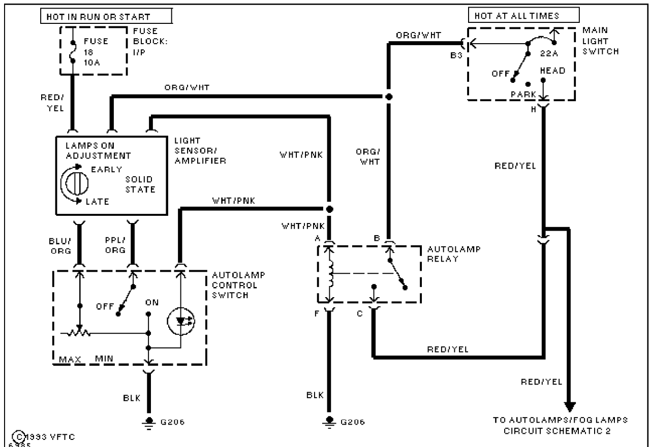
Fig. 52: Autolamps/Fog Lamps (1 of 3)
