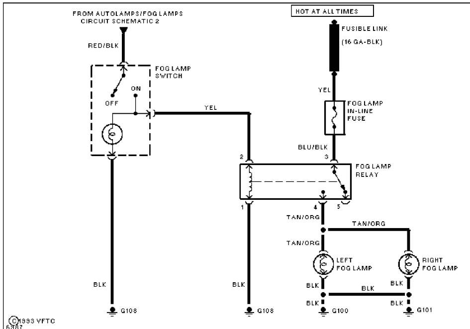
Fig. 54: Autolamps/Fog Lamps (3 of 3)
