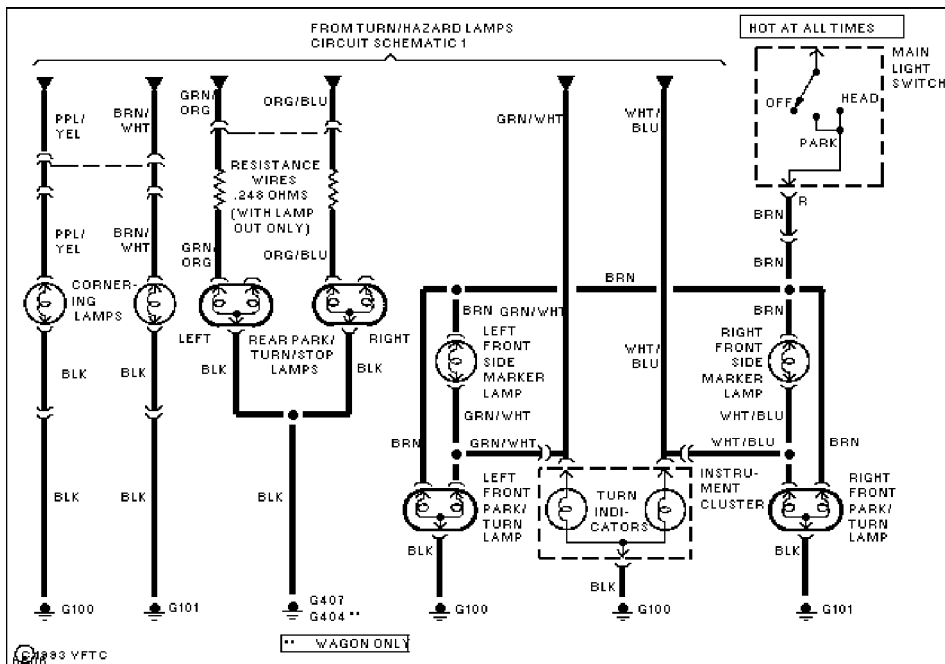
Fig. 51: Turn/Hazard/Stop/Cornering Lamps (1 of 2)
