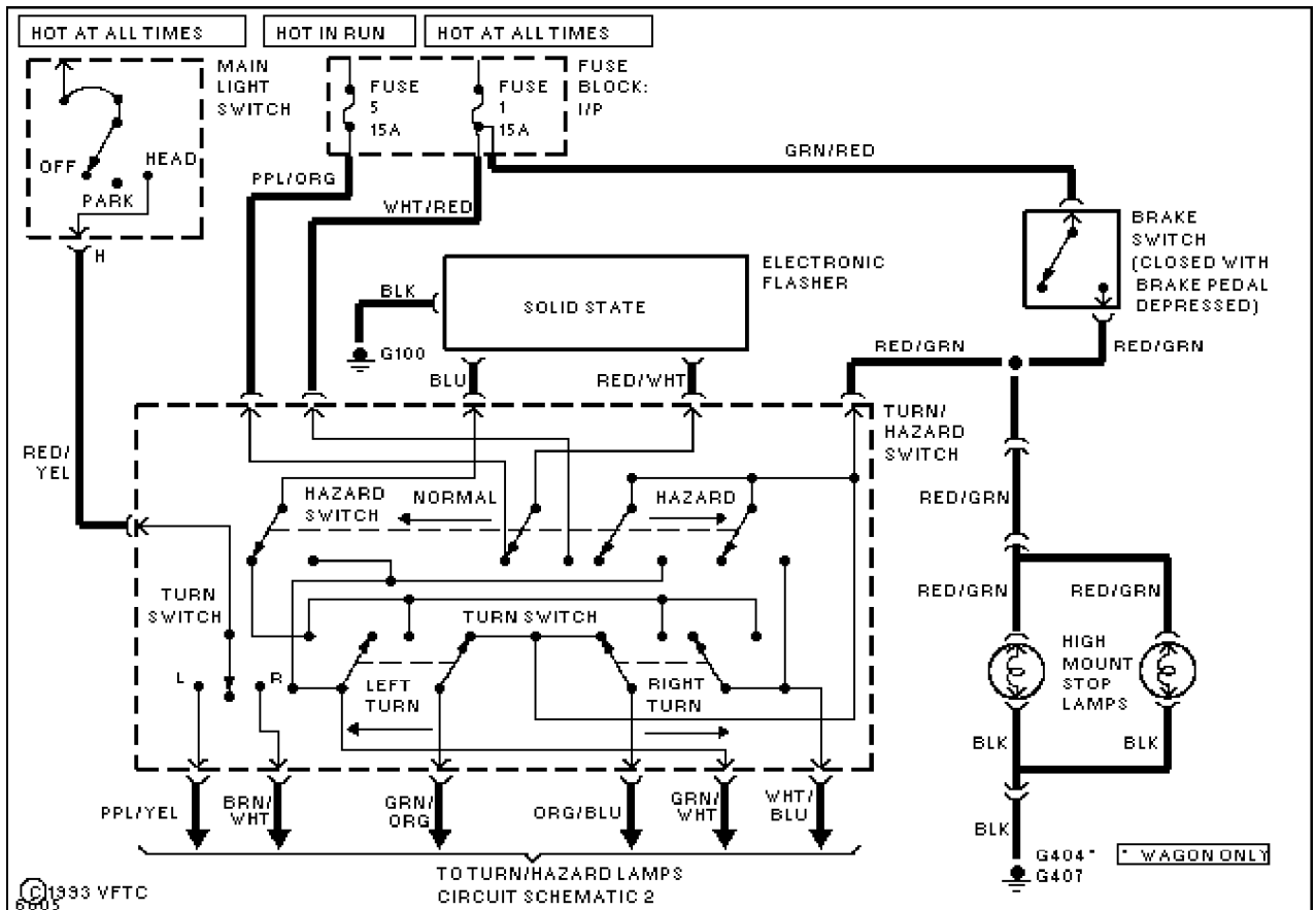
Fig. 50: Turn/Hazard/Stop/Cornering Lamps (1 of 2)
