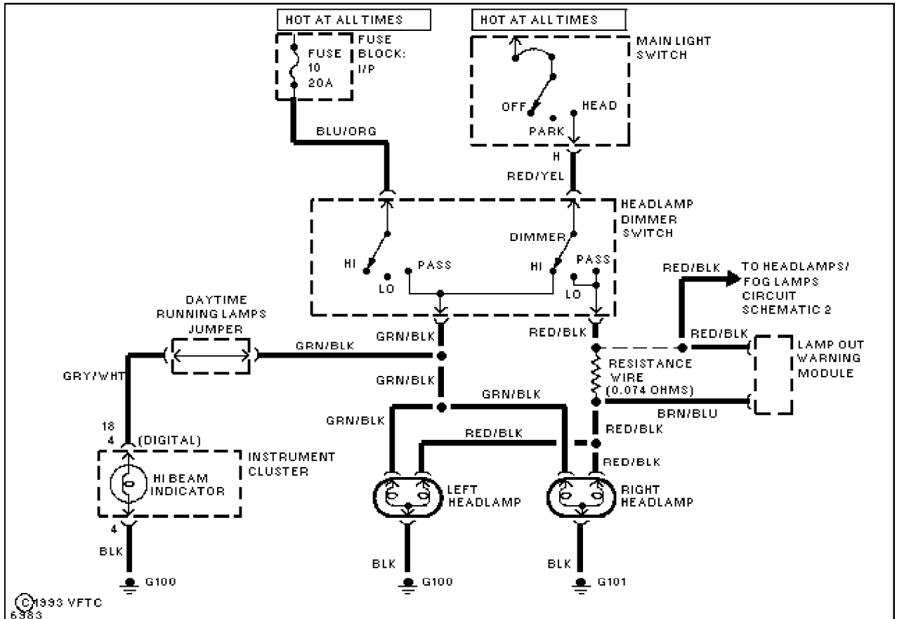
Fig. 55: Headlamps/Fog Lamps (1 of 2)
