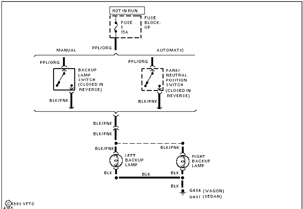
Fig. 47: Backup Lamps
