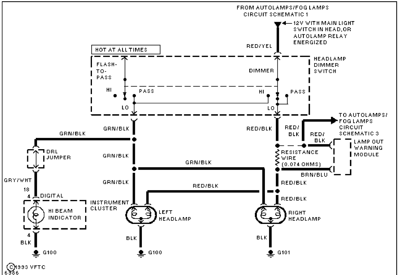
Fig. 53: Autolamps/Fog Lamps (2 of 3)
