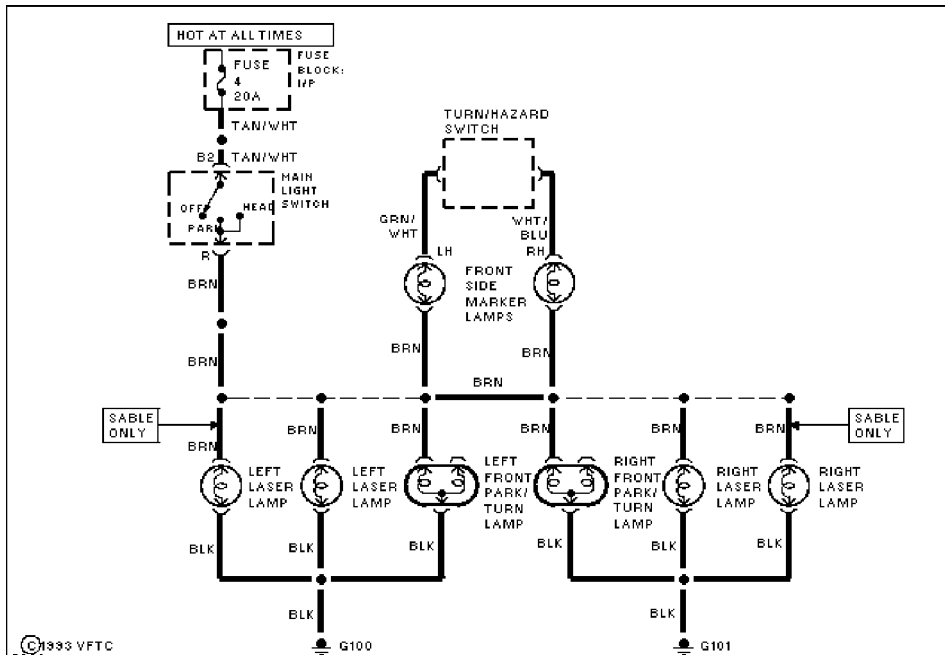
Fig. 49: Park/License Lamps (Sedan W/O Lamp Out Warning) (2 of 2)
