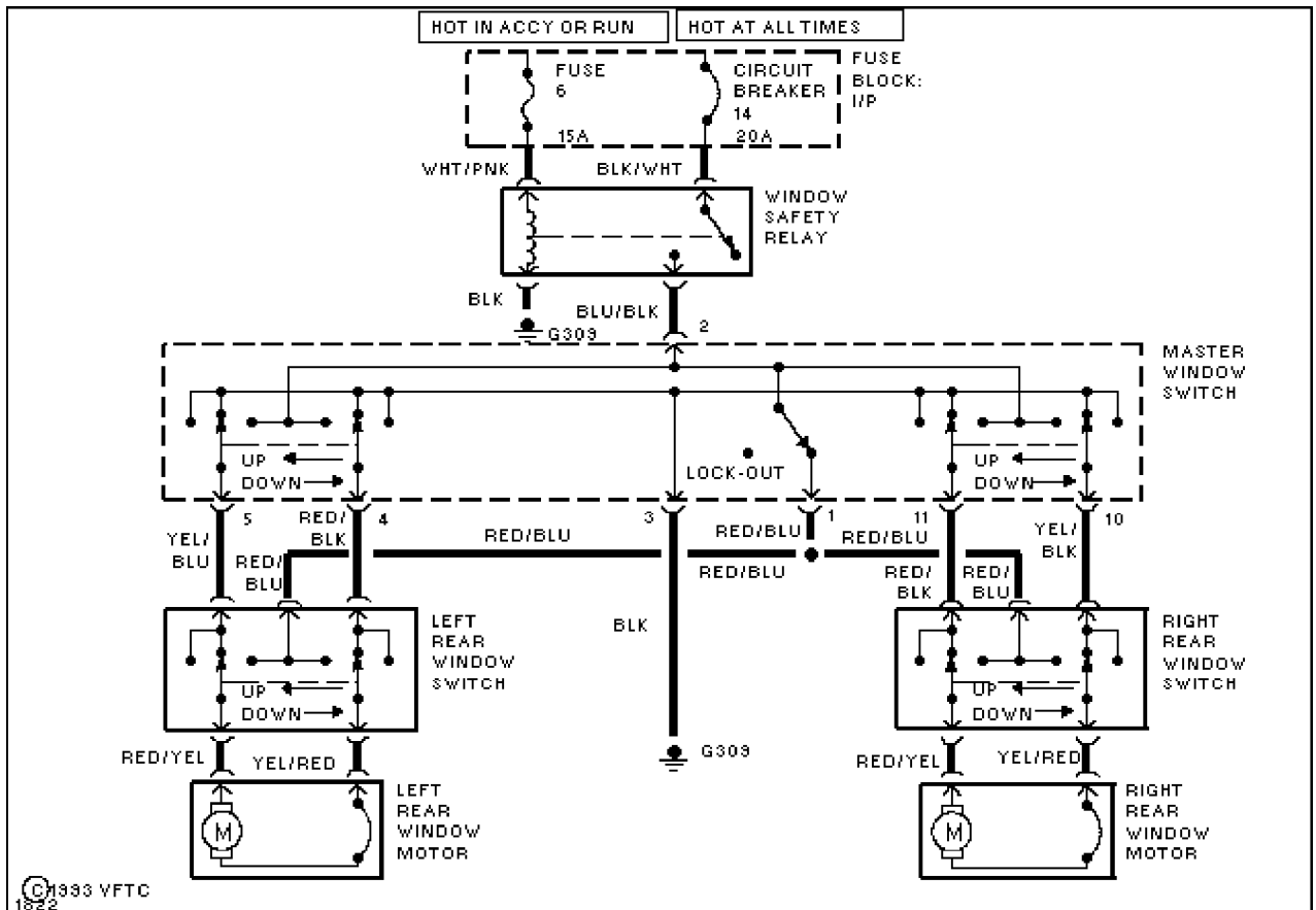
Fig. 73: Power Windows (2 of 2)
