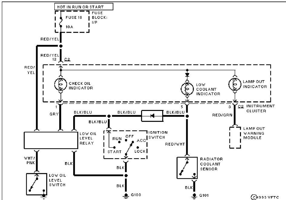
Fig. 69: Electronic Indicators (SHO) (2 of 4)
