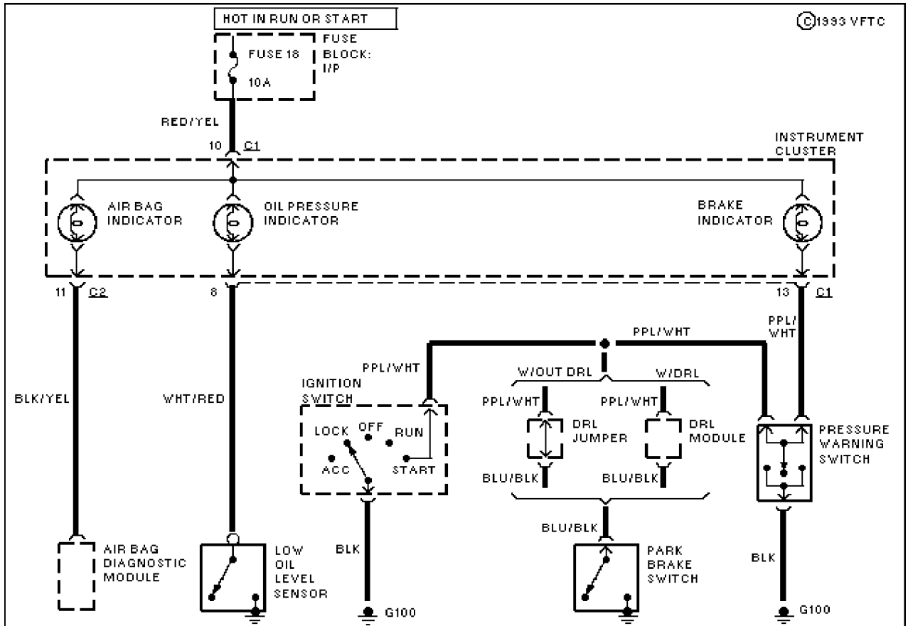
Fig. 68: Electronic Indicators (SHO) (1 of 4)
