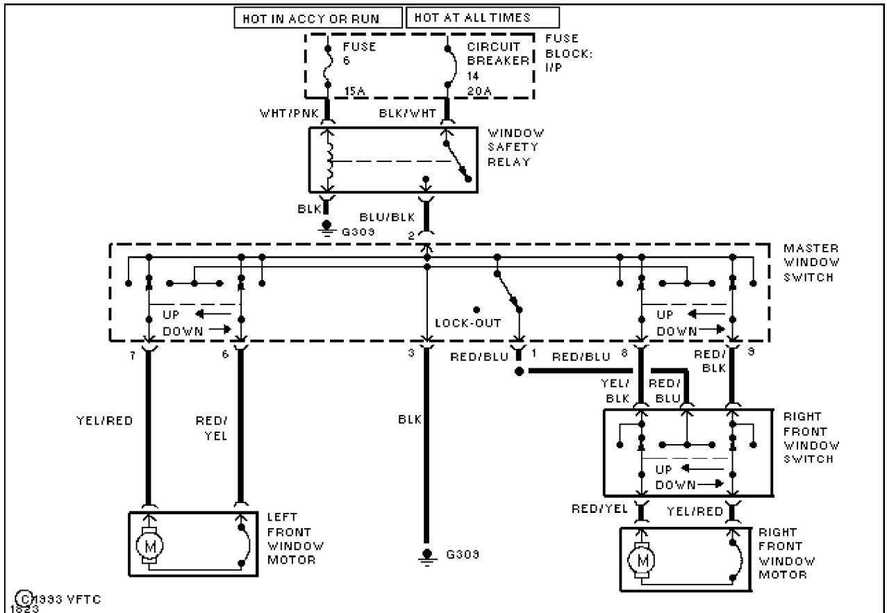
Fig. 72: Power Windows (1 of 2)
