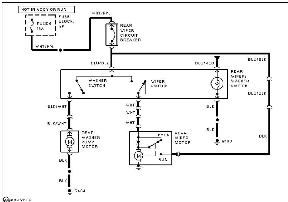
Fig. 82: Rear Wiper/Washer
