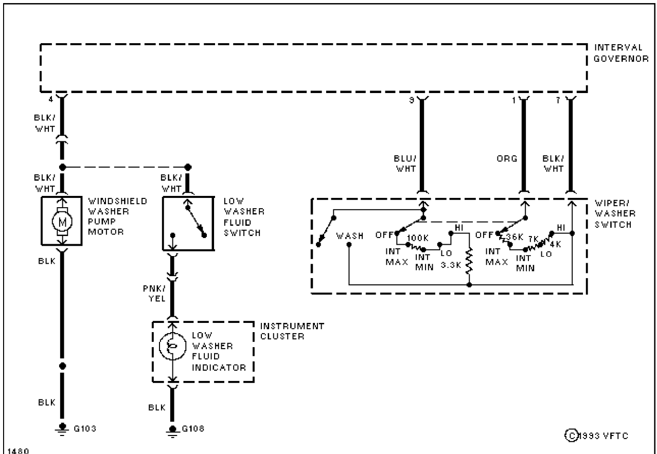
Fig. 81: Interval Wiper/Washer (2 of 2)
