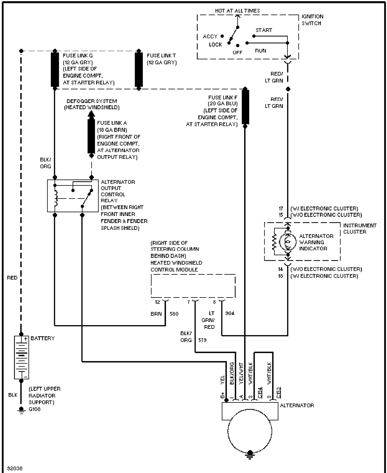
Charging Circuit, W/ Heated Windshield
