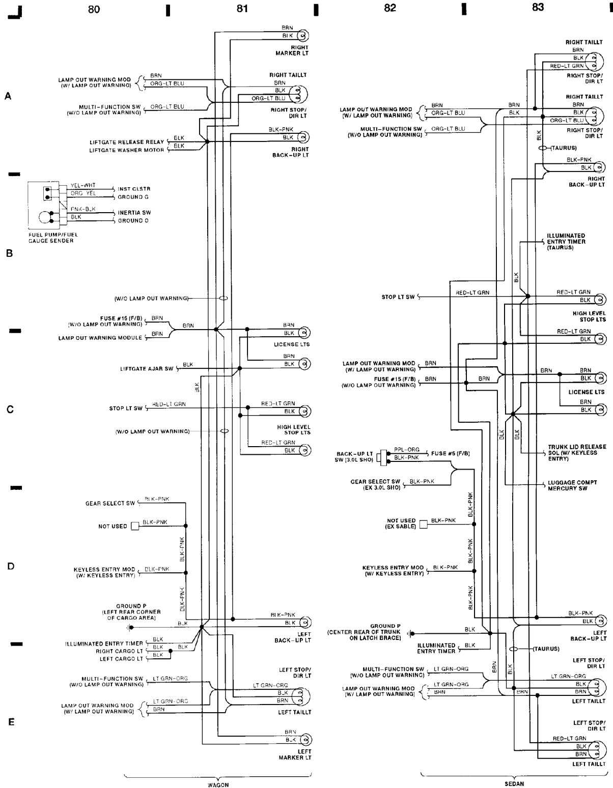
Fig. 21: Taillights (Wagon & Sedan) (Grid 80-83)
