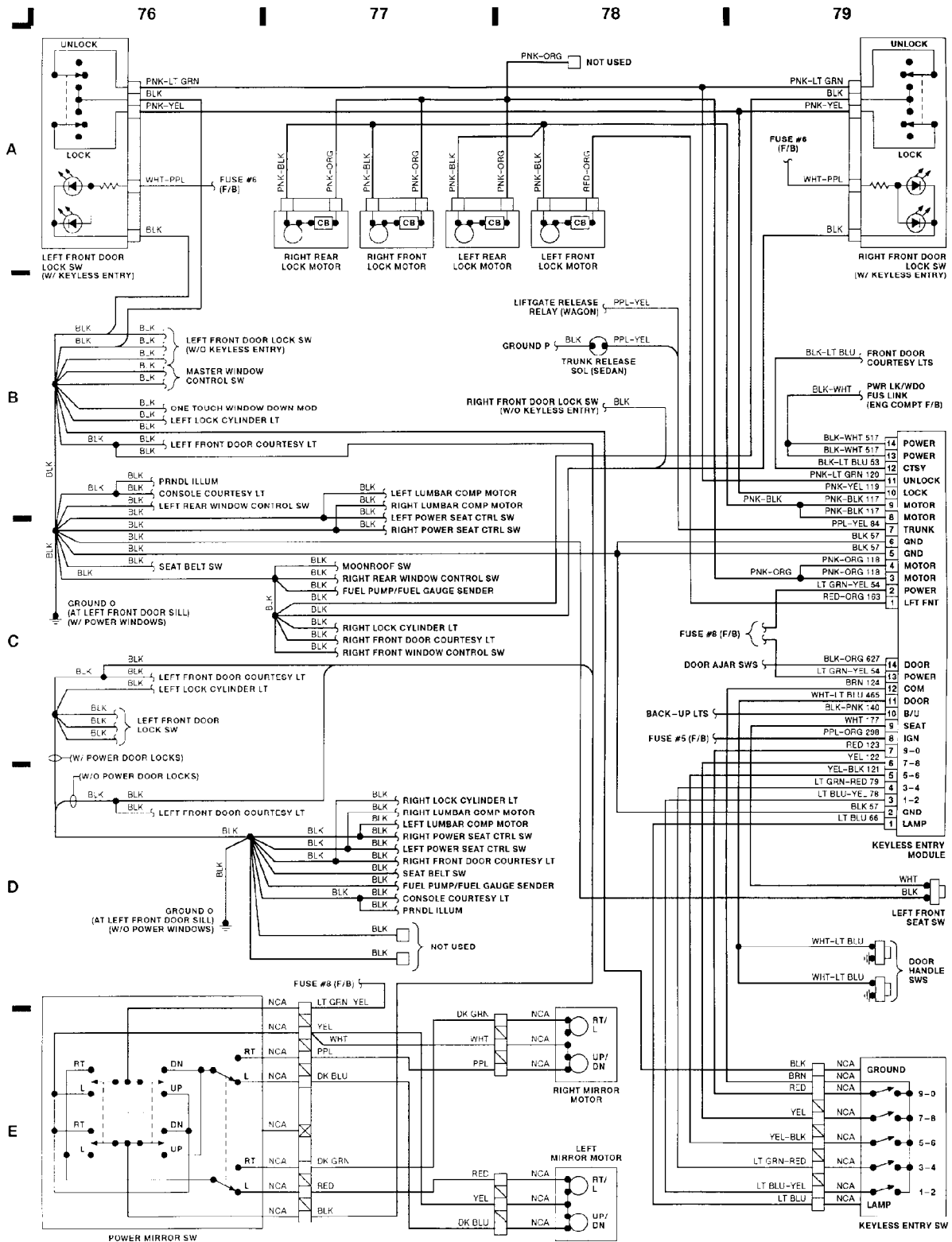
Fig. 20: Power Mirror, Power Doors W/Keyless Entry (Grid 76-79)
