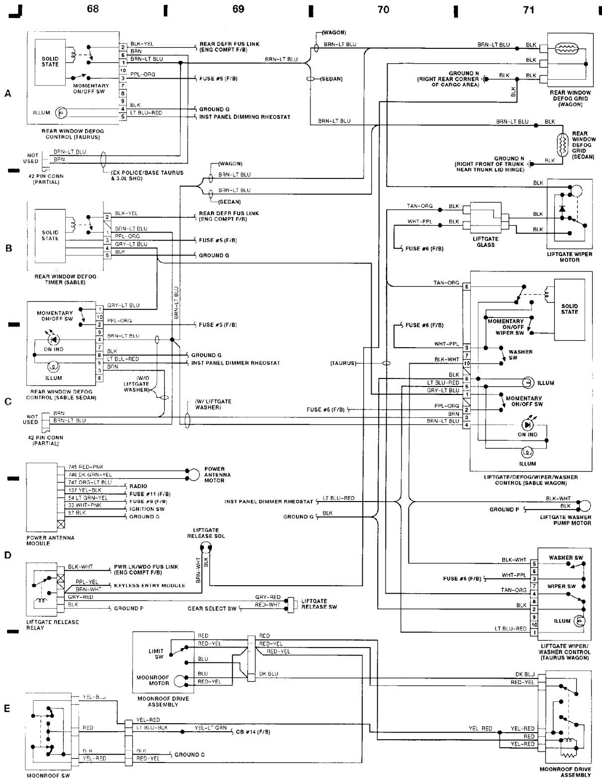
Fig. 18: Power Antenna/Moonroof, Rear Defogger, Liftgate (Grid 68-71)
