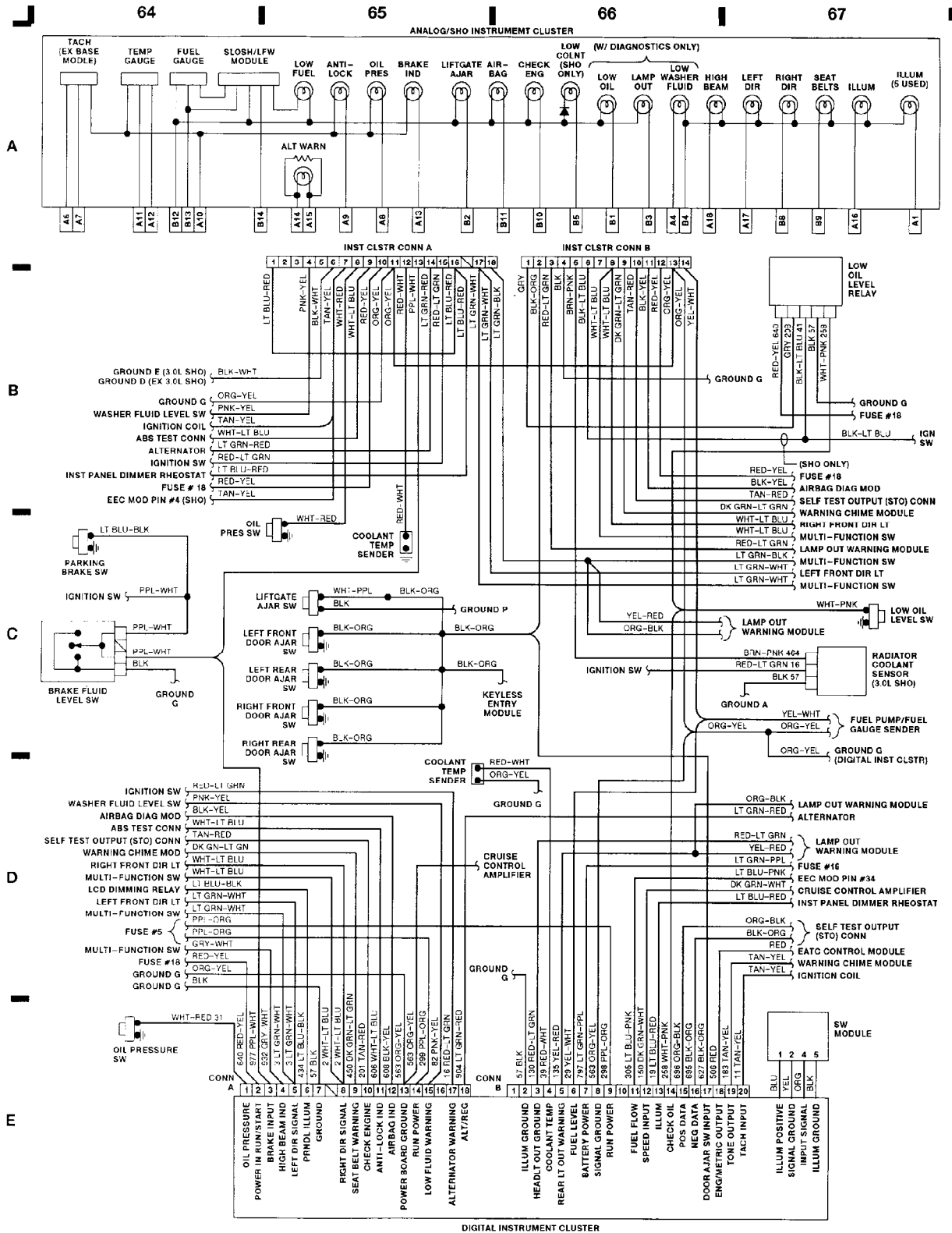
Fig. 17: Analog/SHO & Digital Instrument Panel (Grid 64-67)
