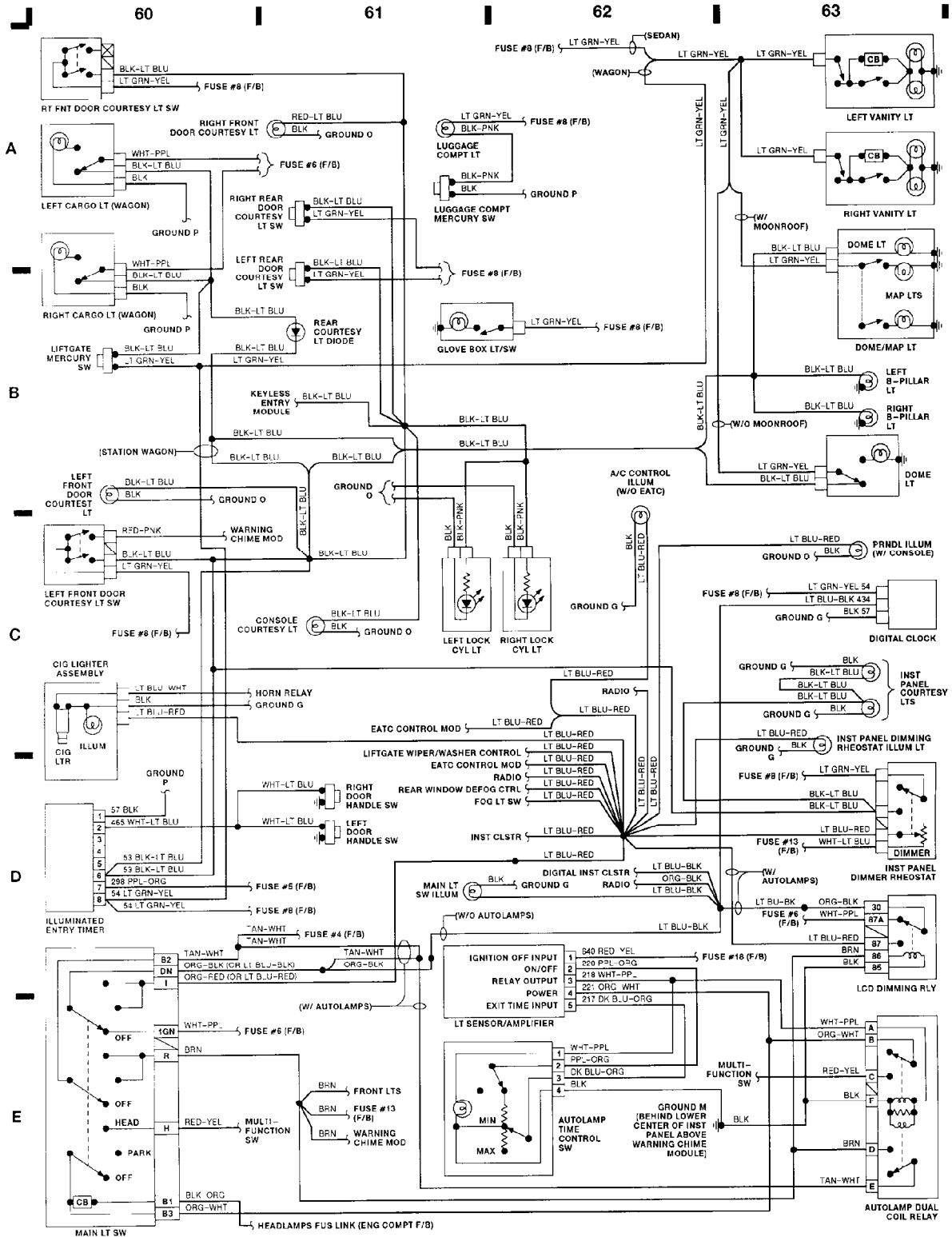
Fig. 16: Main Light Switch, Courtesy Lights (Grid 60-63)
