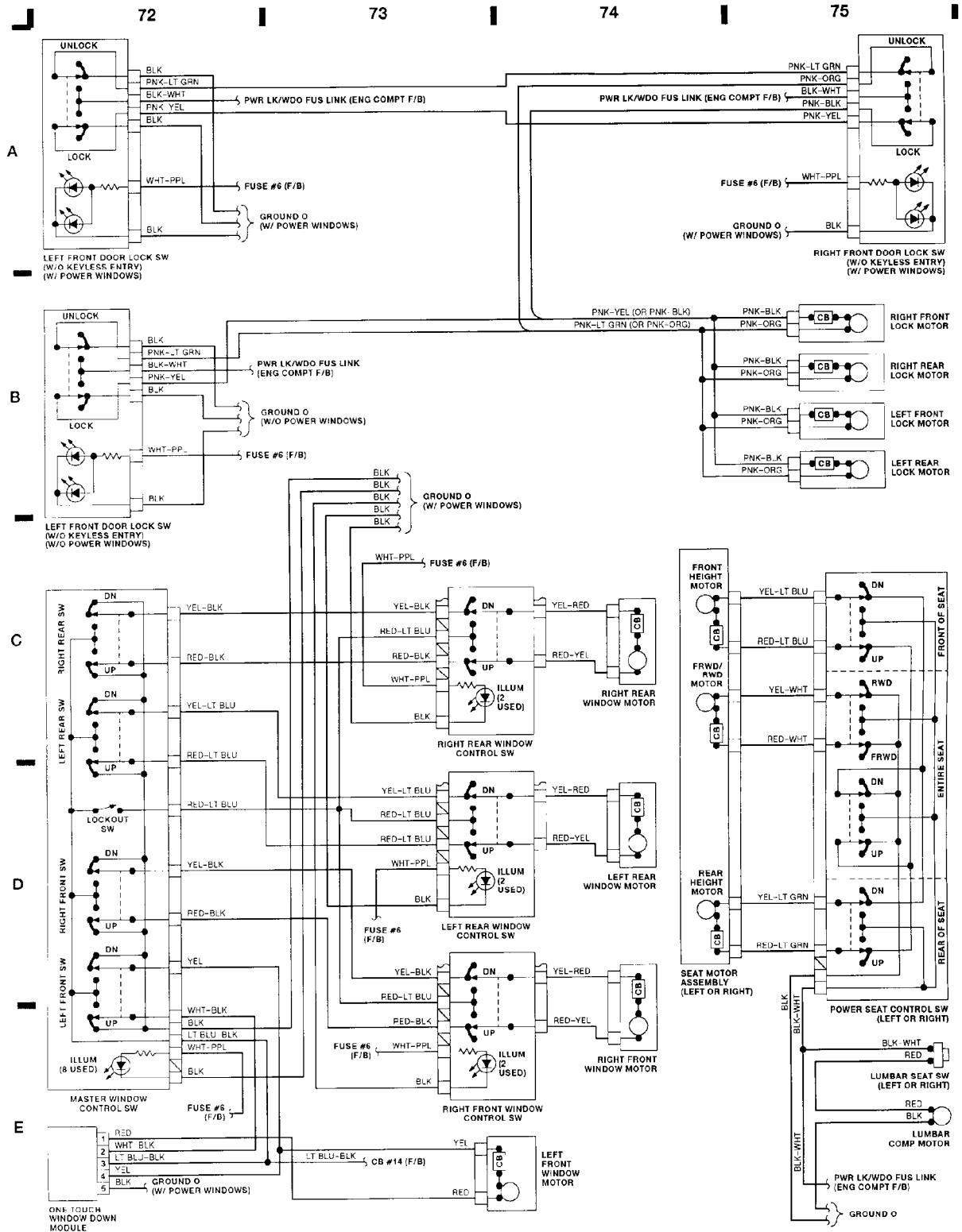
Fig. 19: Pwr Windows/Seats, Pwr Doors W/O Keyless Entry (Grid 72-75)
