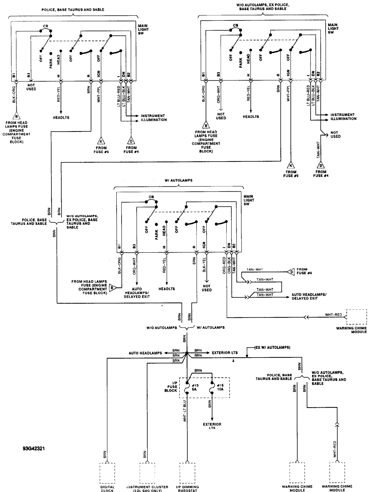
Fig. 14: Power Distribution (6 Of 6)
