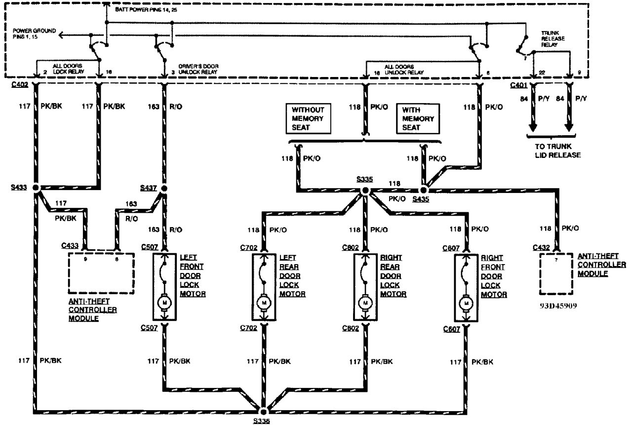
Fig. 58: Remote Keyless Entry With Power Door Locks (4 Of 5)
