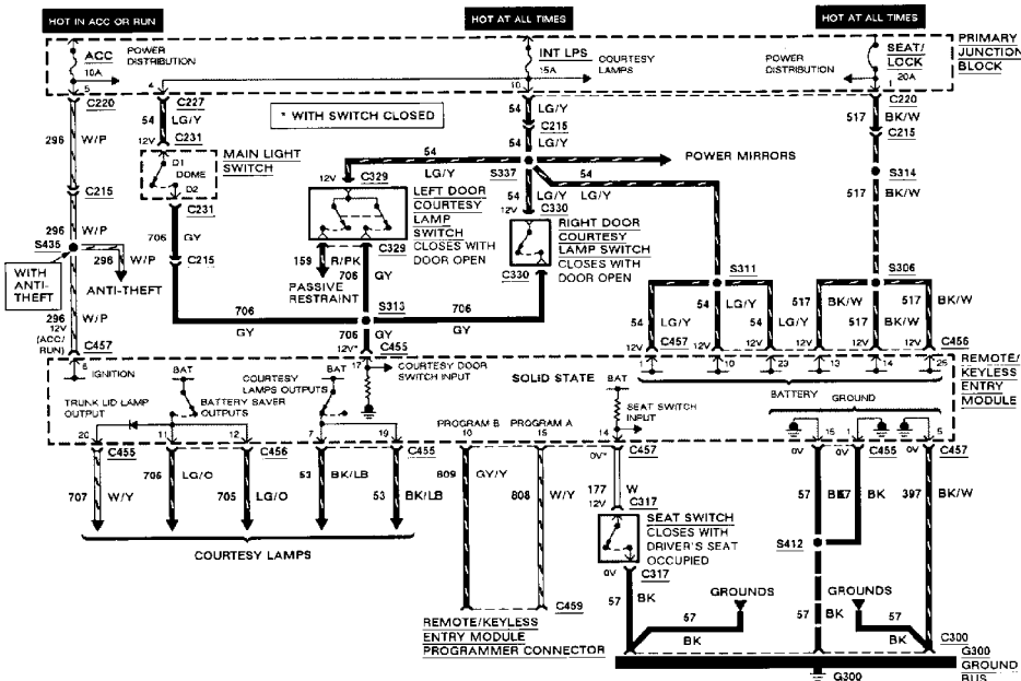
Fig. 61: Remote Keyless Entry Wiring Diagram (2 Of 4)
