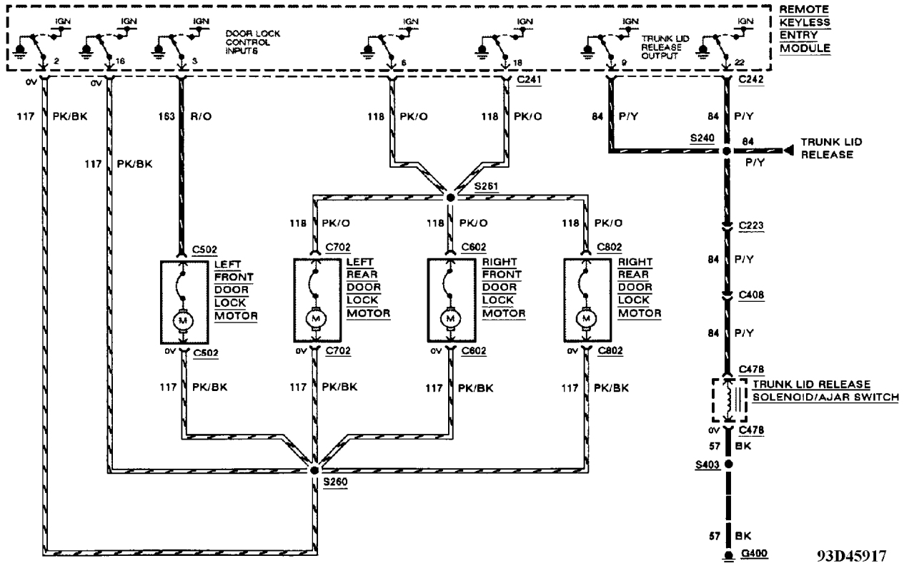
Fig. 66: Remote Keyless Entry With Illuminated Entry (3 Of 4)
