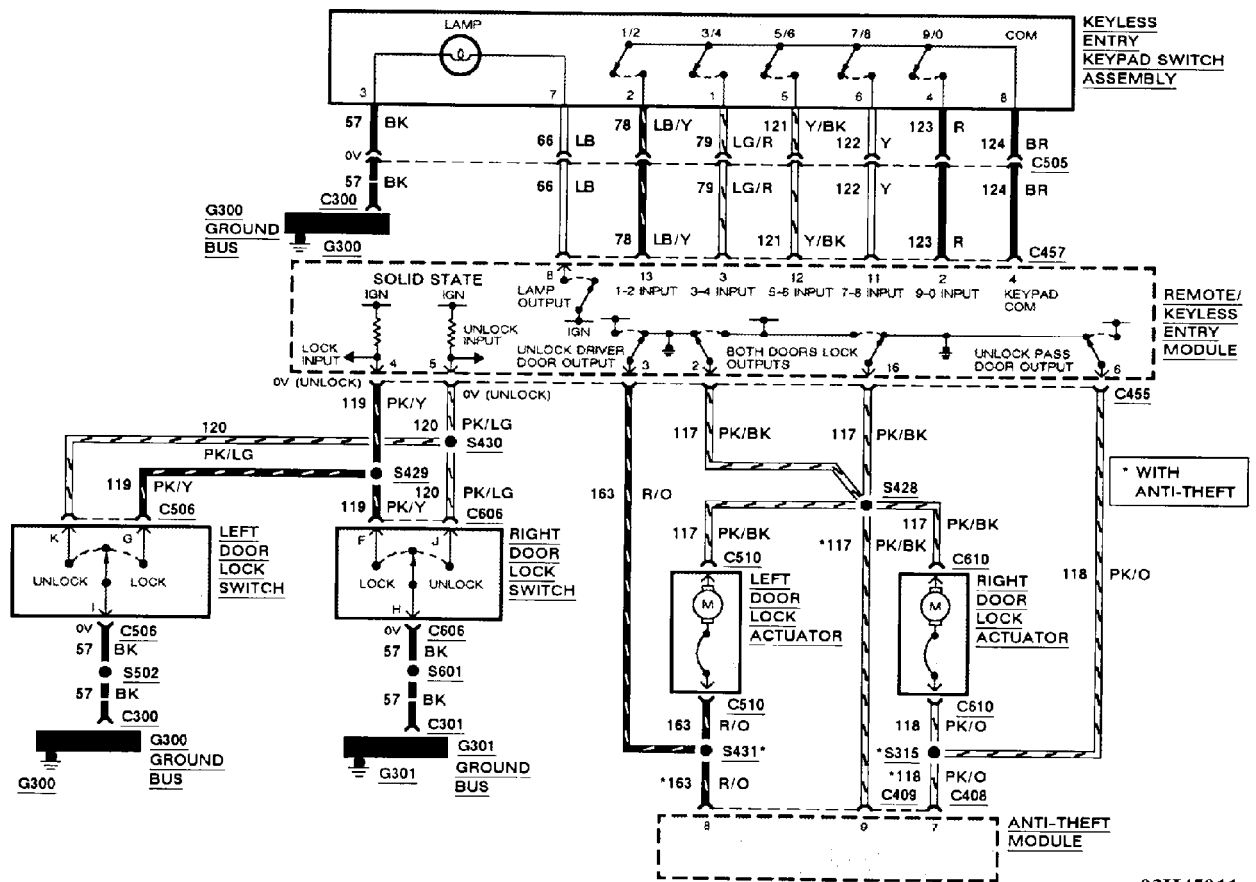
Fig. 60: Remote Keyless Entry Wiring Diagram (1 Of 4)
