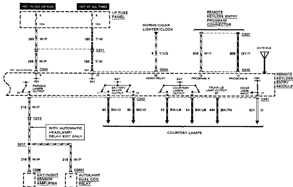
Fig. 65: Remote Keyless Entry With Illuminated Entry (2 Of 4)
