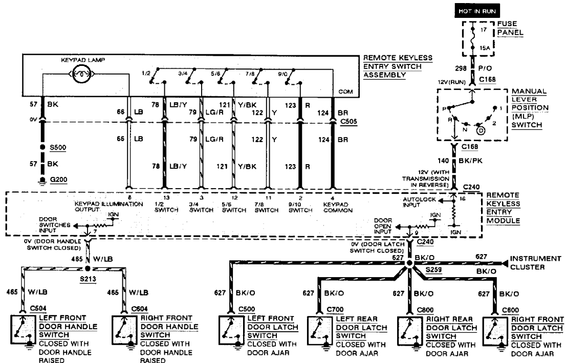
Fig. 67: Remote Keyless Entry With Illuminated Entry (4 Of 4)
