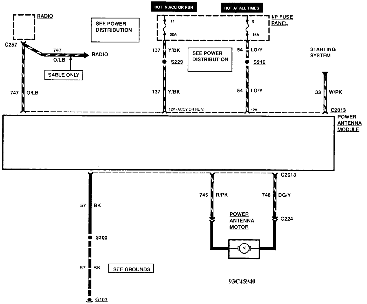
Fig. 73: Power Antenna Wiring Diagram
