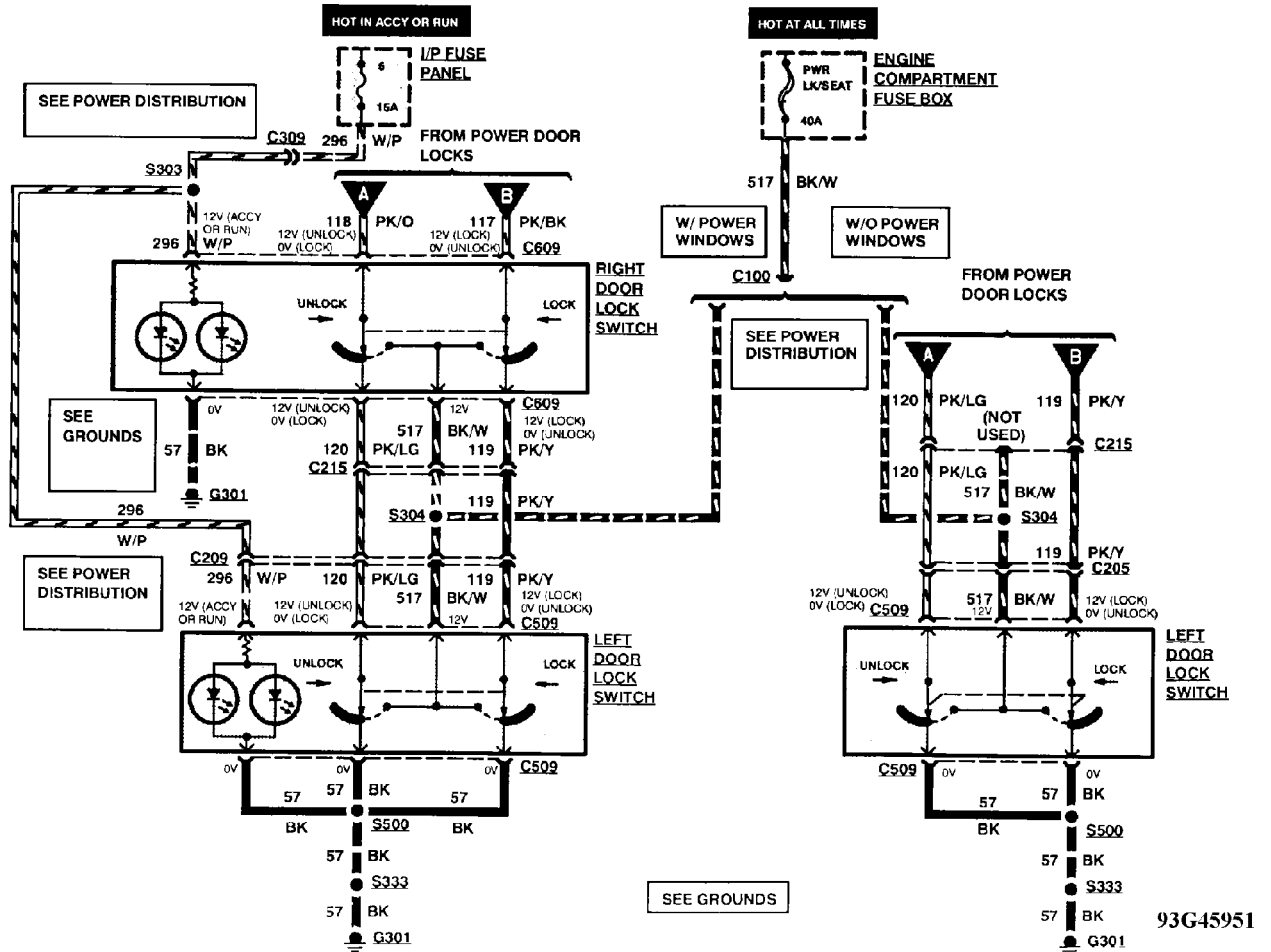
Fig. 74: Power Door Locks Wiring Diagram (1 Of 2)
