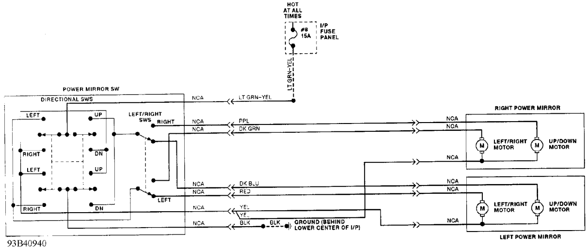
Fig. 76: Power Mirror System Wiring Diagram
