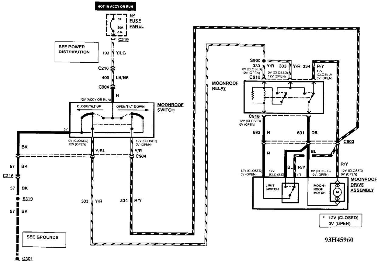
Fig. 77: Power Moon Roof Wiring Diagram
