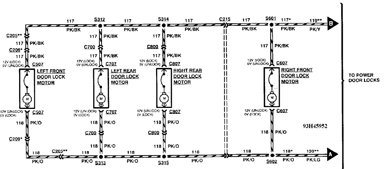
Fig. 75: Power Door Locks Wiring Diagram (2 Of 2)
