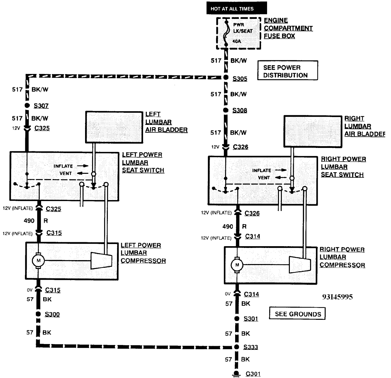
Fig. 78: Lumbar Seat Wiring Diagram
