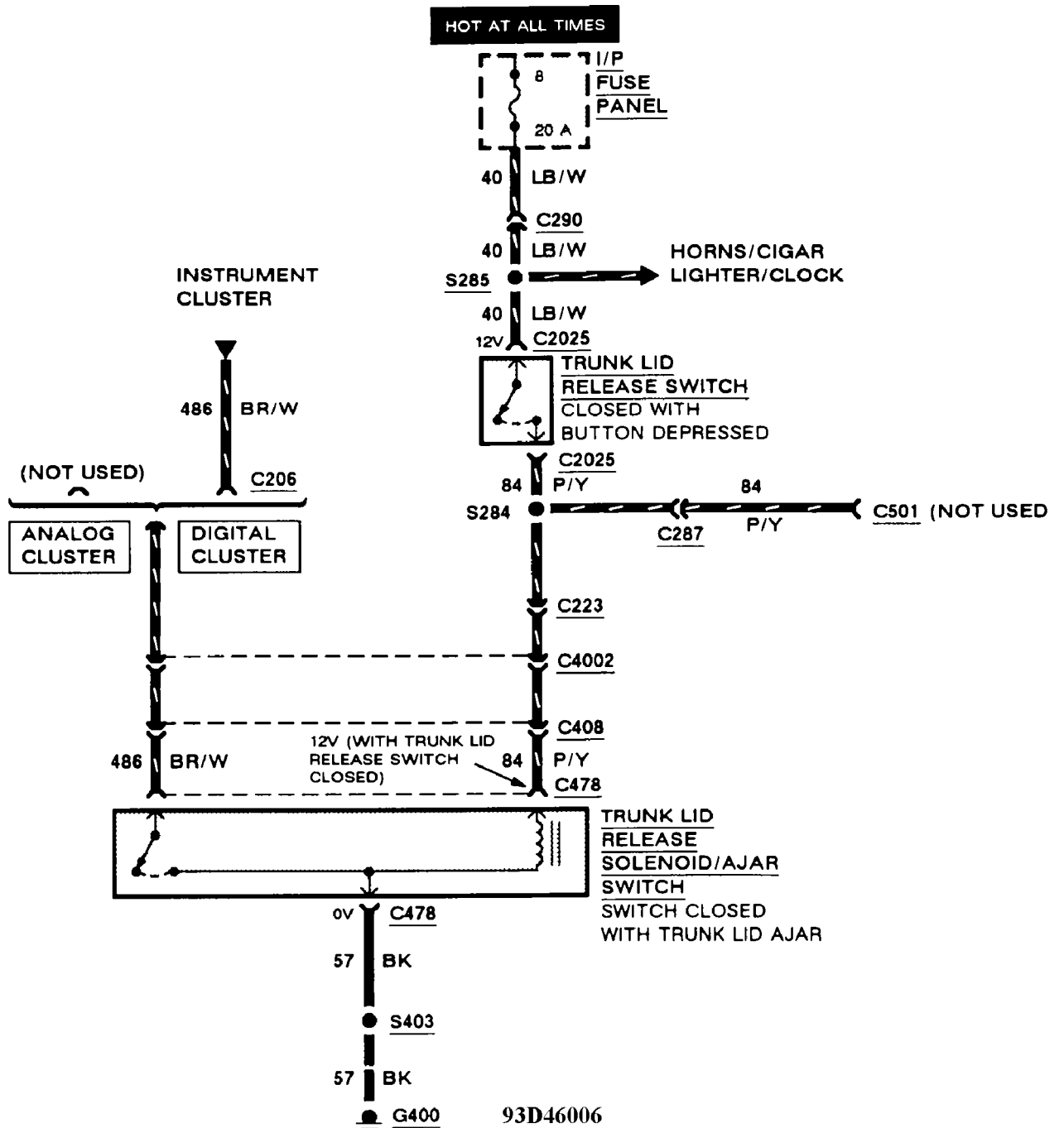
Fig. 83: Power Trunk Release W/ Police Package Wiring Diagram
