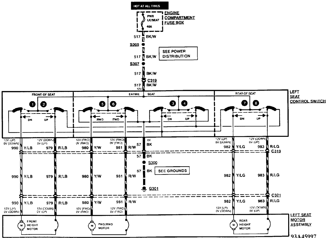
Fig. 80: Power Seats (2 Of 2)
