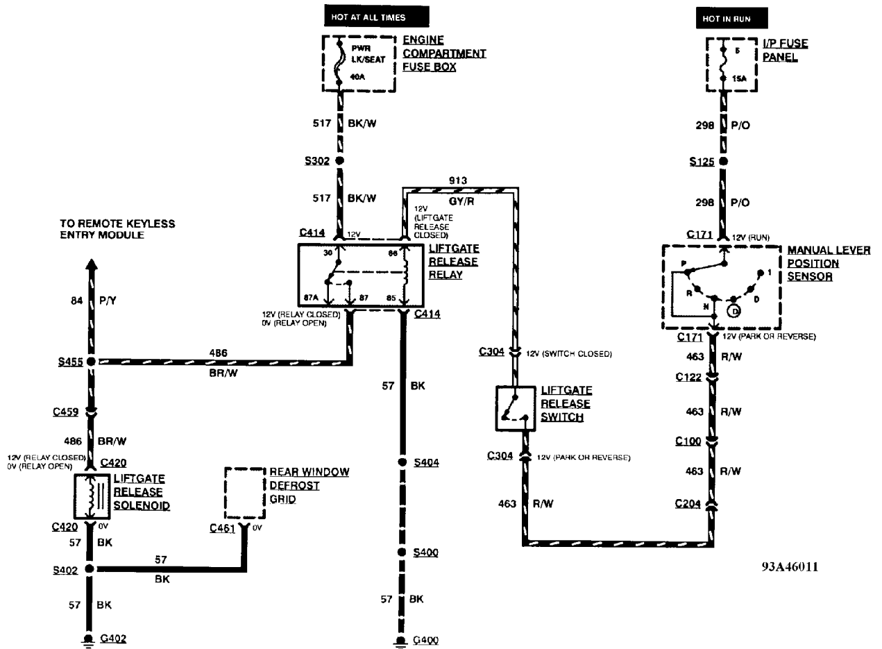
Fig. 85: Power Liftgate Release Wiring Diagram
