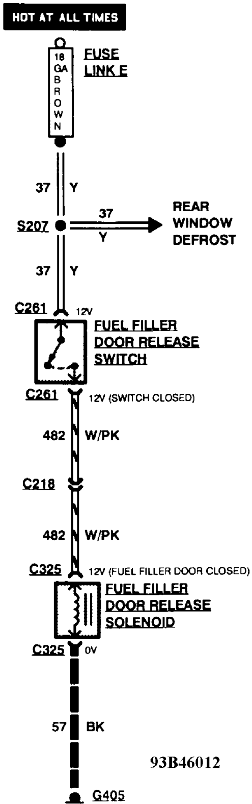
Fig. 86: Power Fuel Filler Door Release Wiring Diagram
