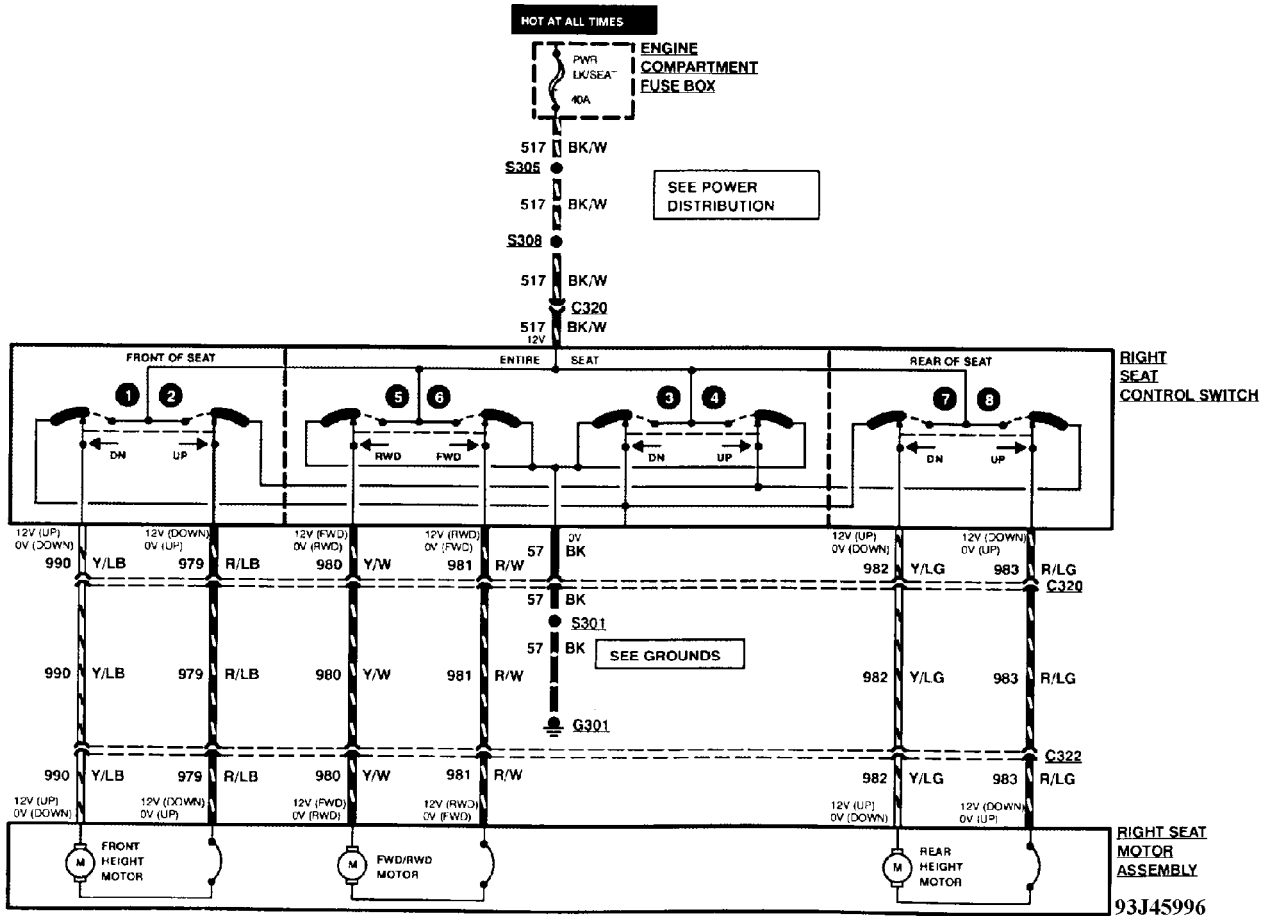
Fig. 79: Power Seats (1 Of 2)
