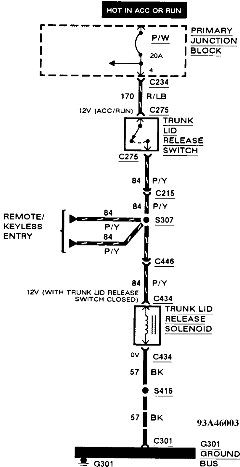
Fig. 81: Power Fuel Filler Door Release Wiring Diagram (1 Of 2)
