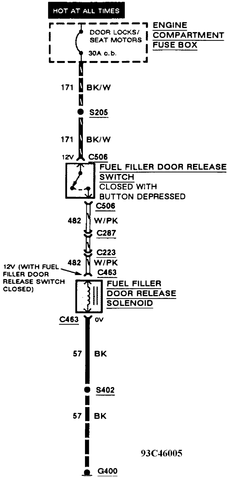
Fig. 82: Power Fuel Filler Door Release Wiring Diagram (2 Of 2)
