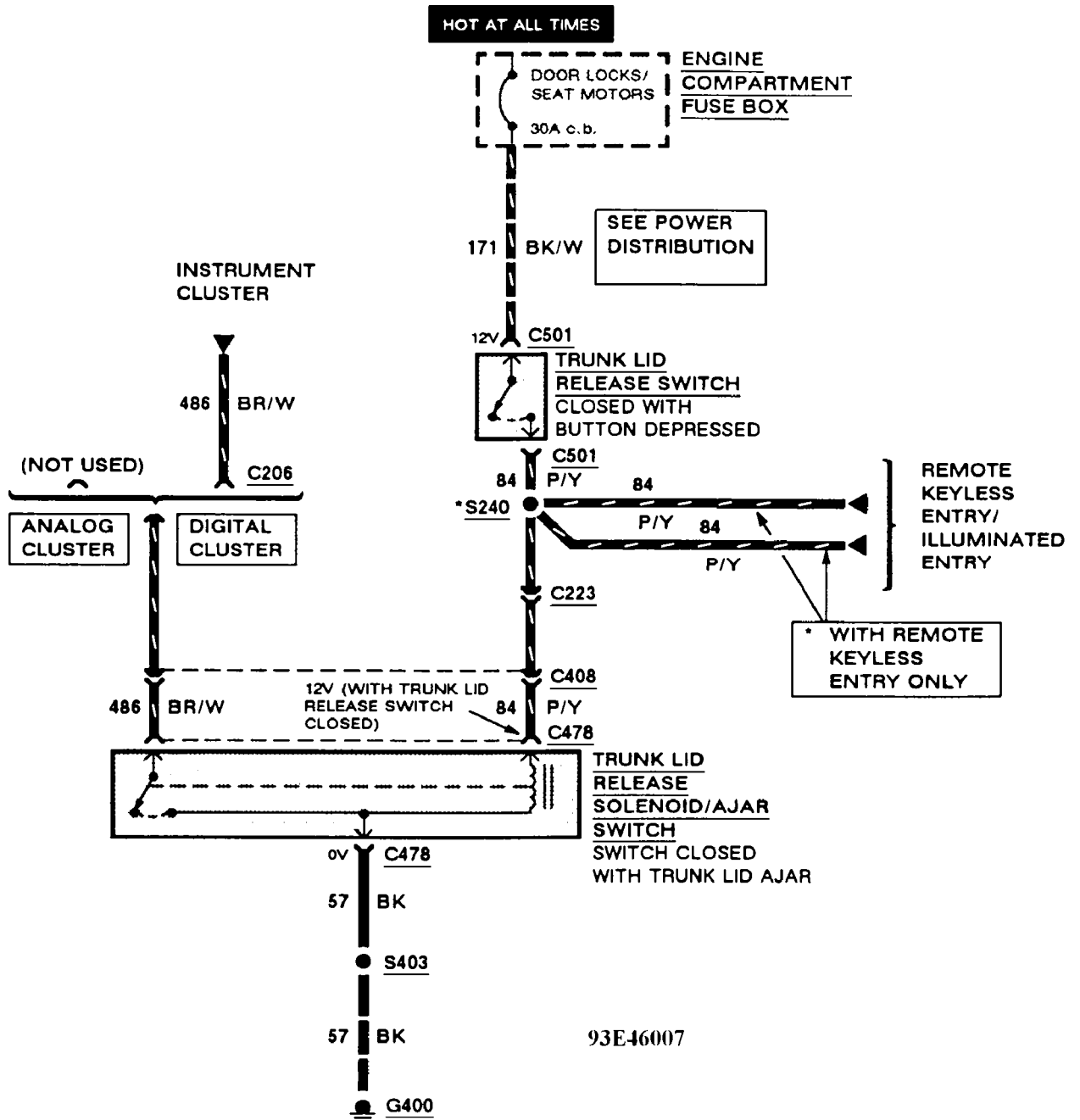
Fig. 84: Power Trunk Release W/O Police Package Wiring Diagram
