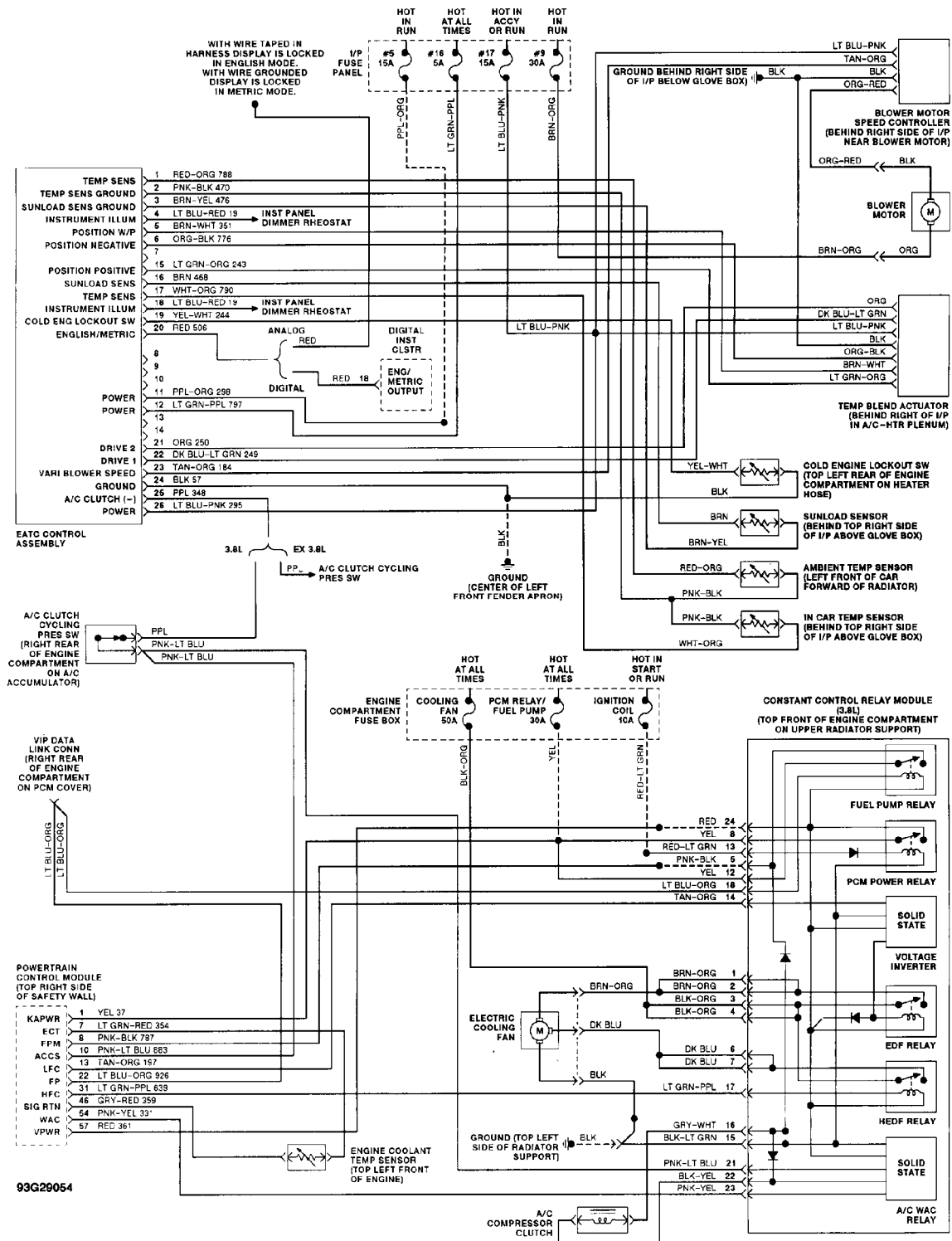
Fig. 94: Auto A/C-Heater Sys Wiring Diagram (1 Of 4)
