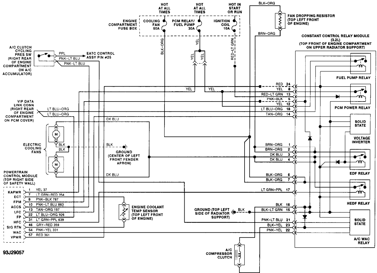
Fig. 97: Auto A/C-Heater Sys Wiring Diagram (4 Of 4)
