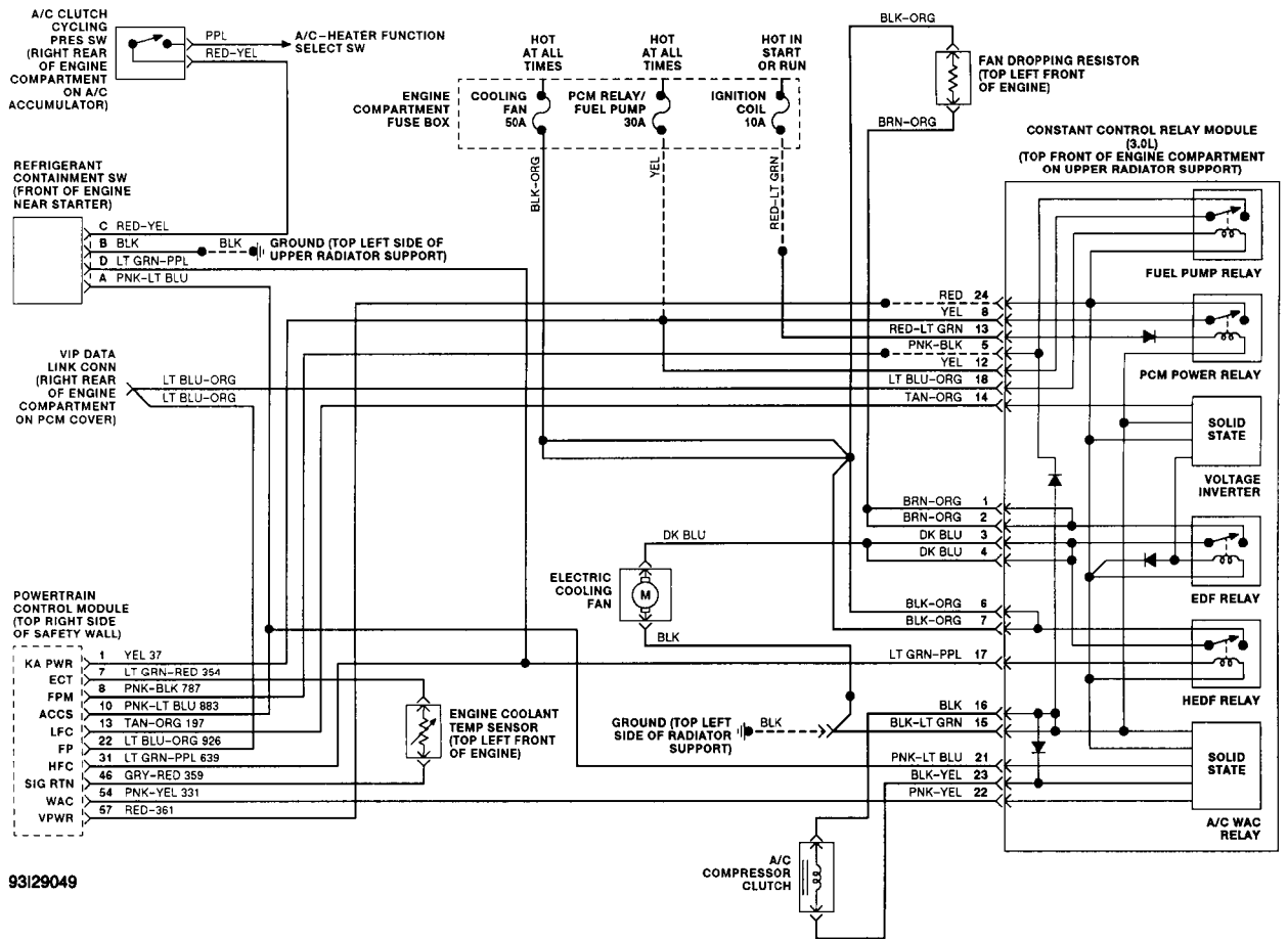
Fig. 101: Man. A/C-Heater Sys. Wiring Diagram (3 Of 4)
