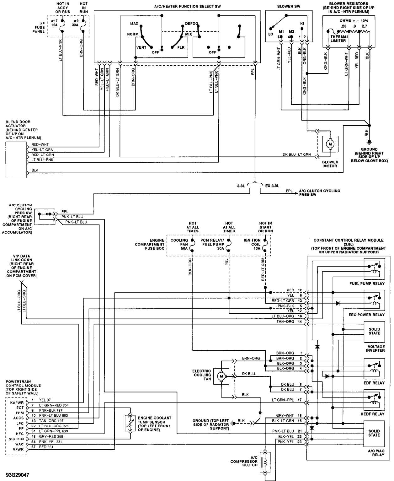
Fig. 99: Man. A/C-Heater Sys. Wiring Diagram (1 Of 4)
