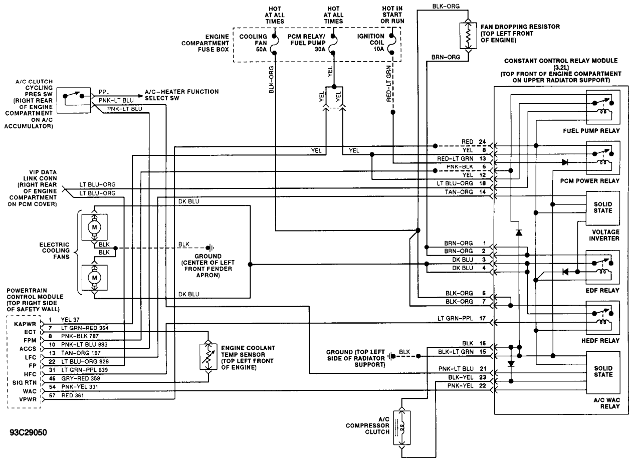
Fig. 102: Man. A/C-Heater Sys. Wiring Diagram (4 Of 4)
