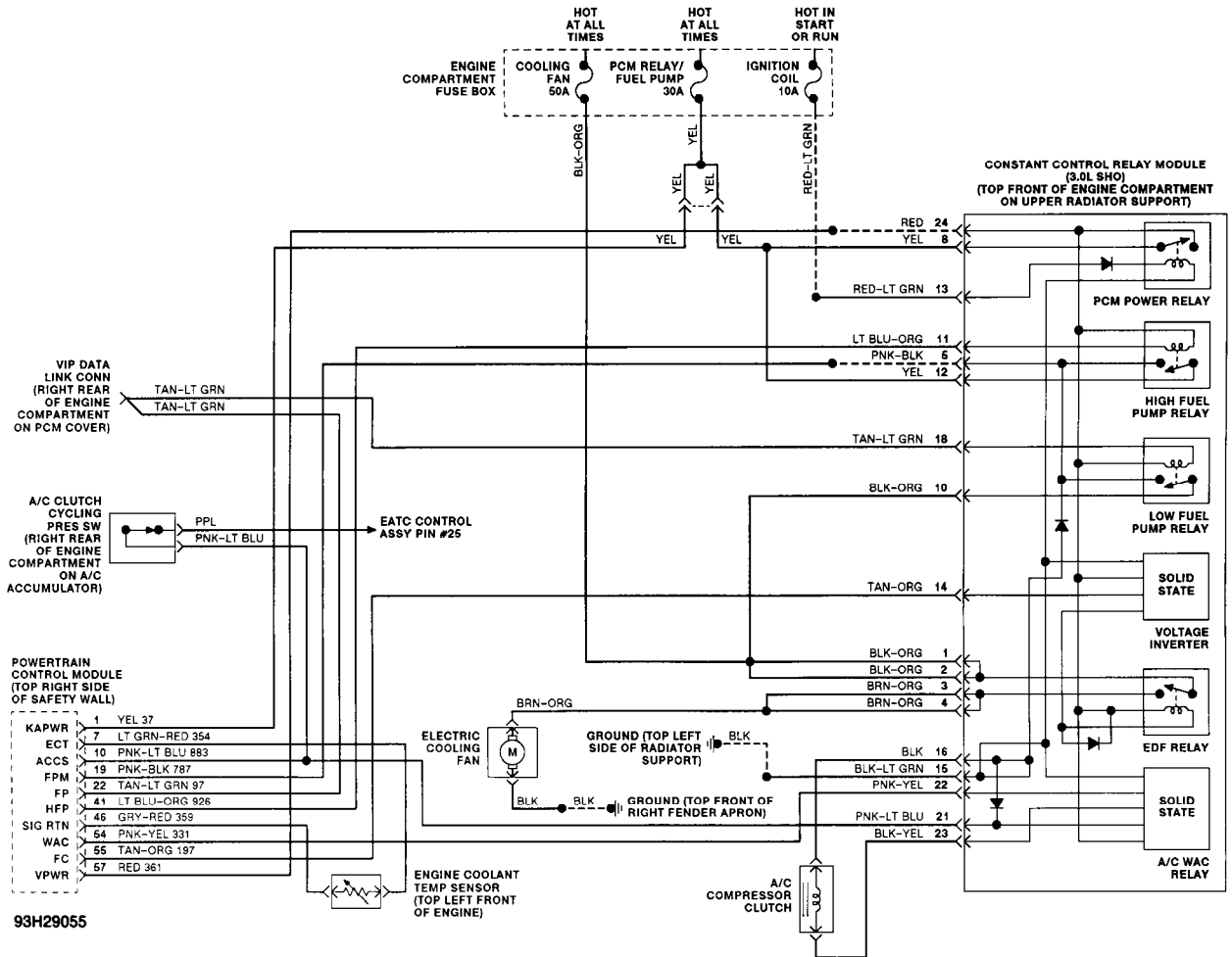
Fig. 95: Auto A/C-Heater Sys Wiring Diagram (2 Of 4)
