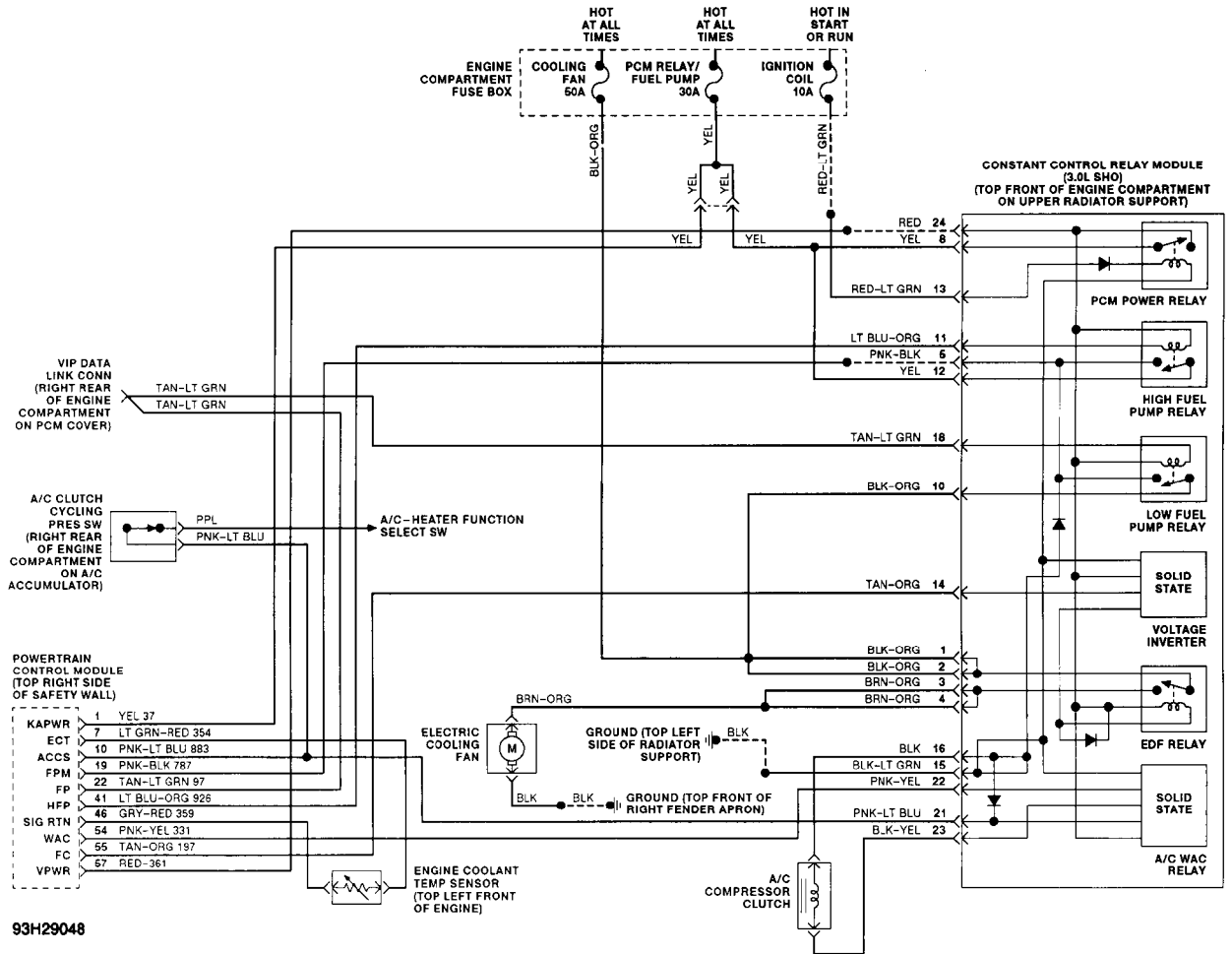
Fig. 100: Man. A/C-Heater Sys. Wiring Diagram (2 Of 4)
