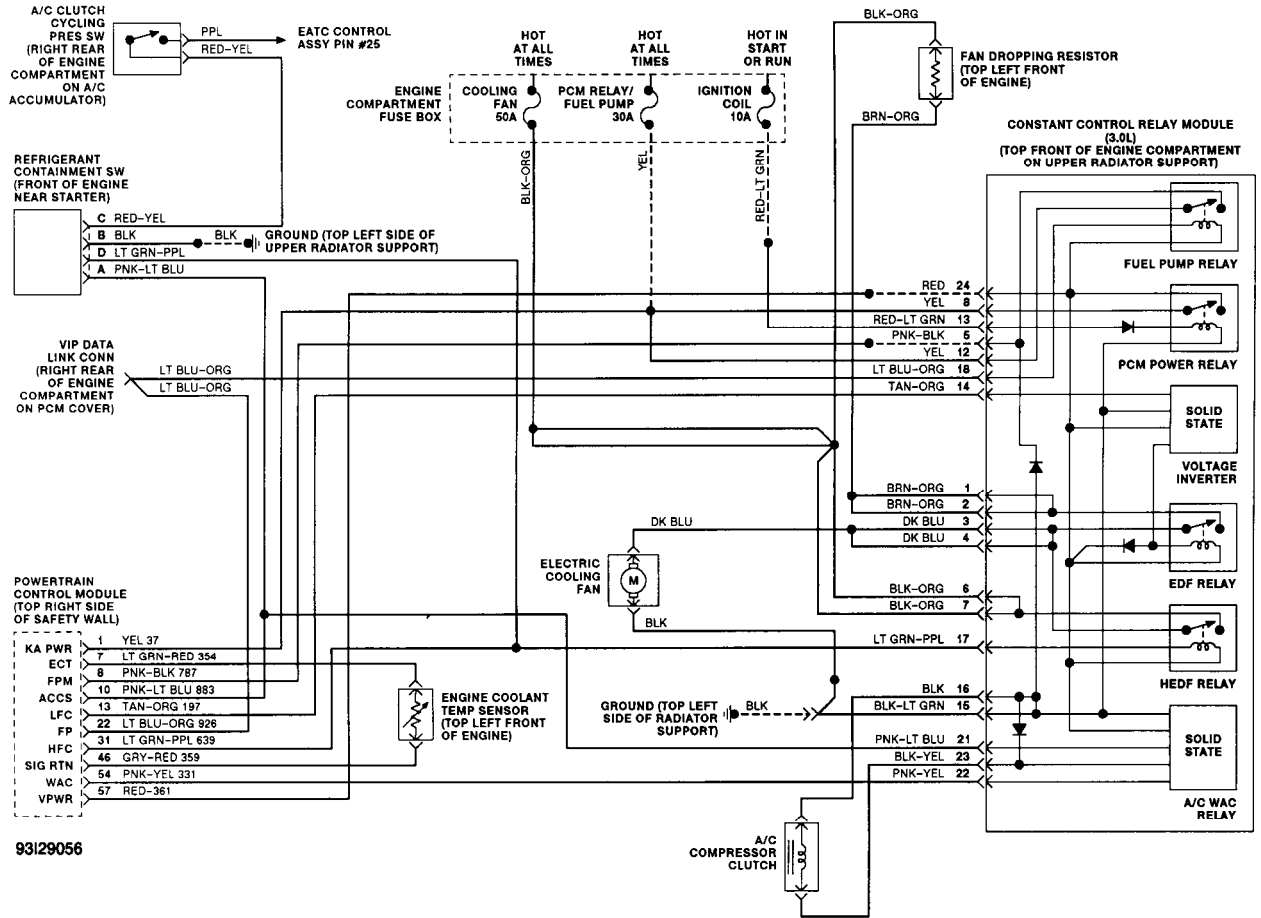
Fig. 96: Auto A/C-Heater Sys Wiring Diagram (3 Of 4)
