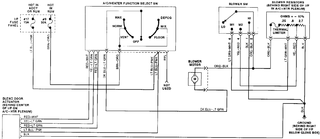
Fig. 98: Heater System Wiring Diagram
