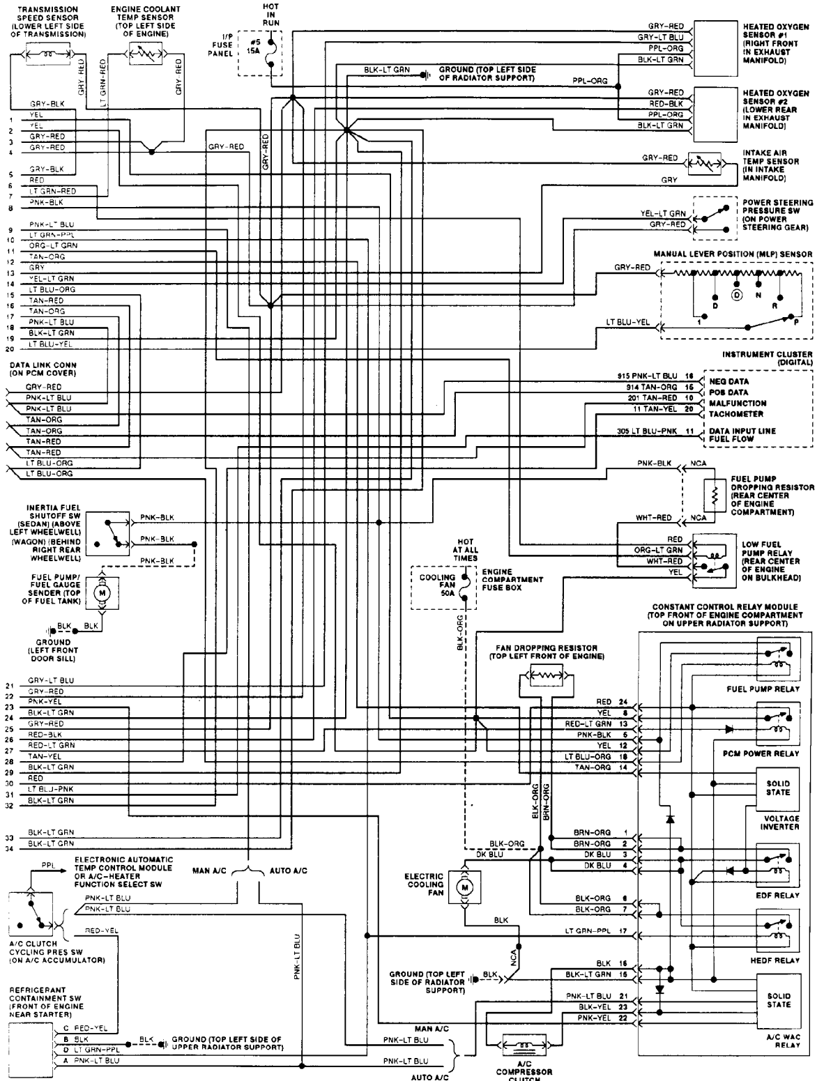
Fig. 125: EEC-IV Wiring Diagram (3.0L Flex Fuel - 2 of 2)
