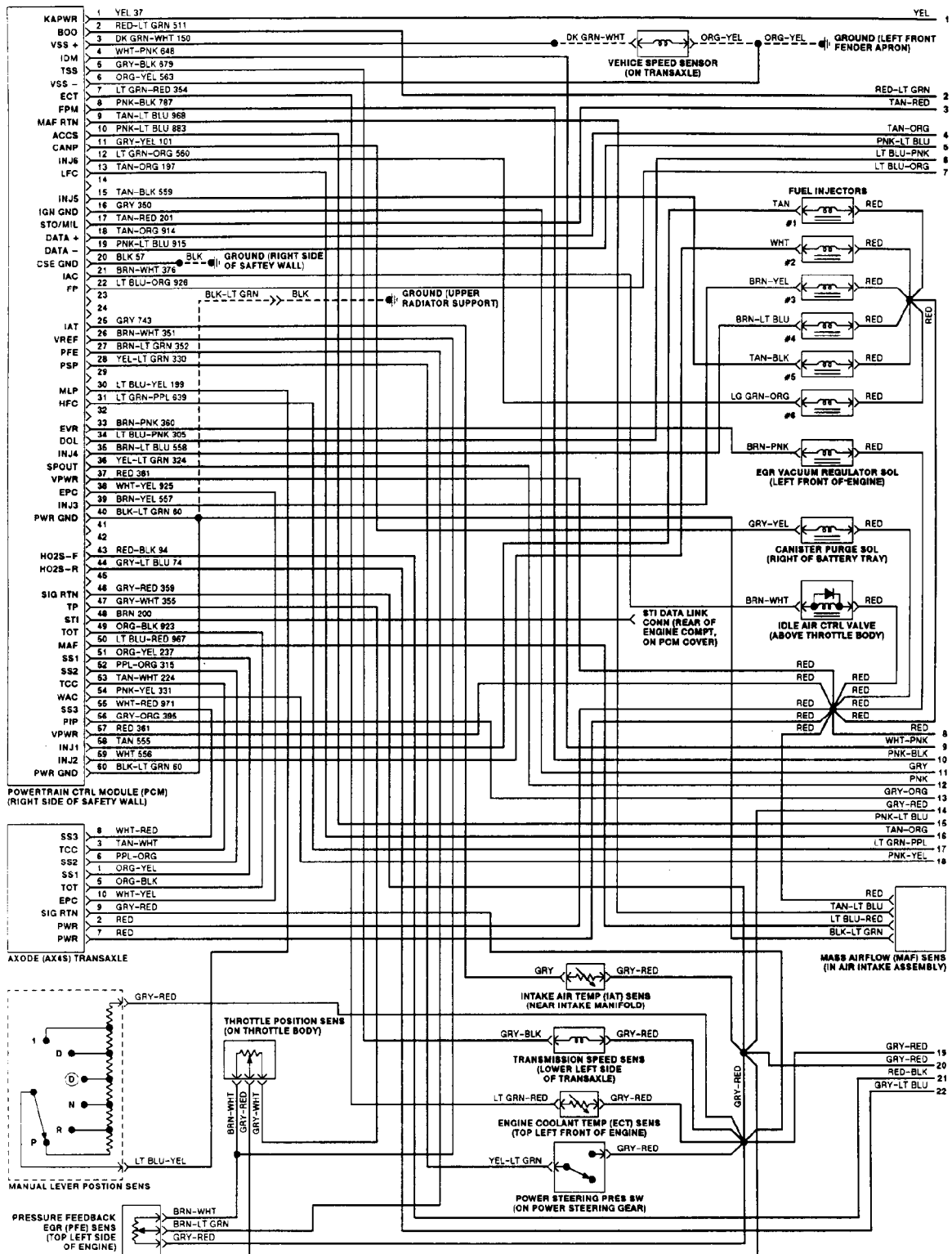
Fig. 122: EEC-IV Wiring Diagram (3.8L - 1 of 2)
