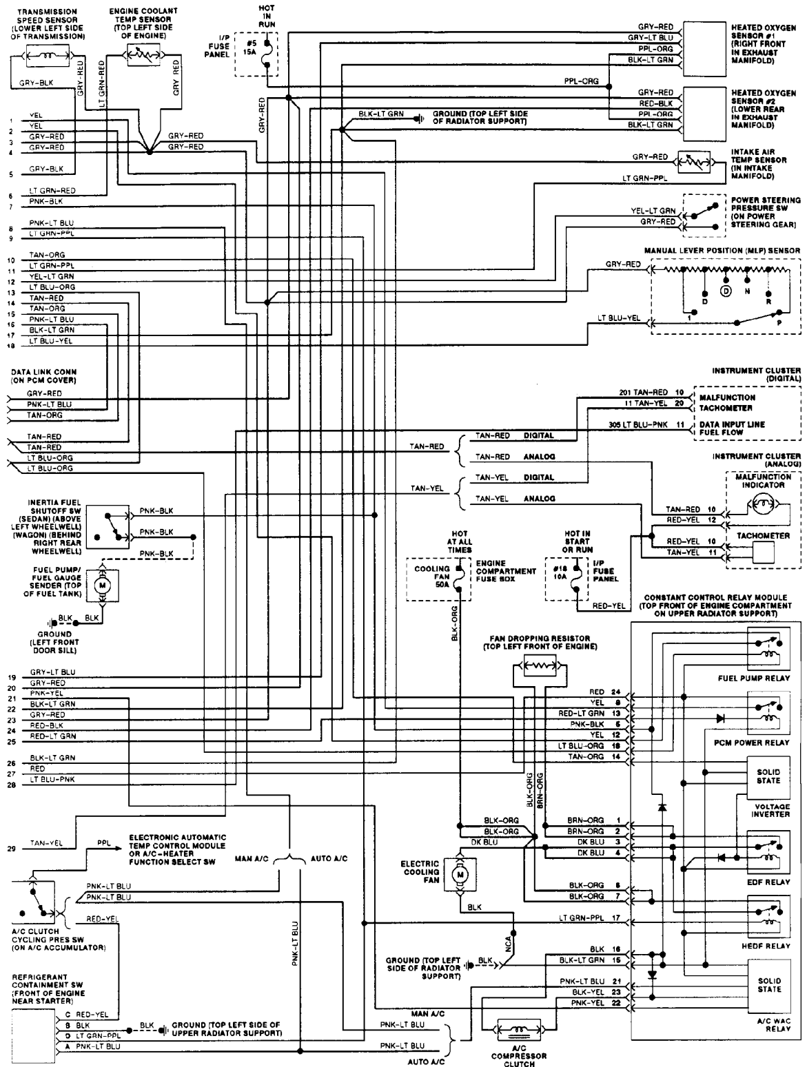
Fig. 121: EEC-IV Wiring Diagram (3.0L Except SHO 2 of 2)
