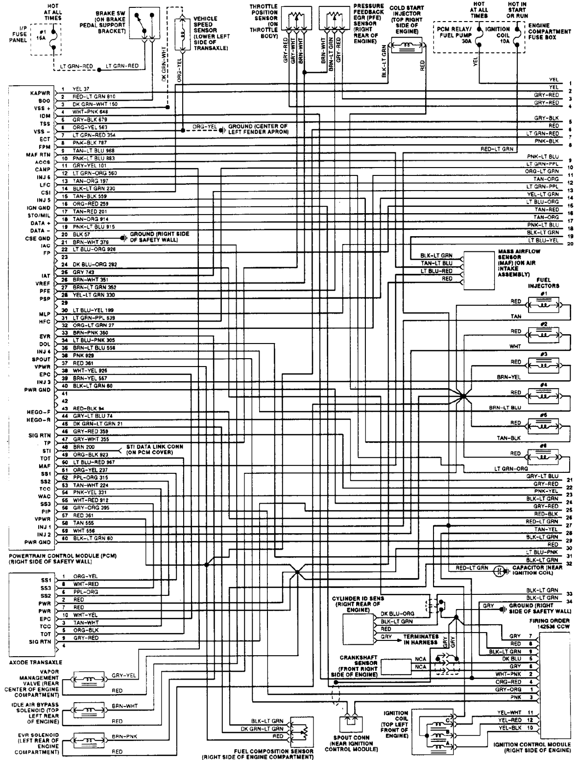
Fig. 124: EEC-IV Wiring Diagram (3.0L Flex Fuel - 1 of 2)
