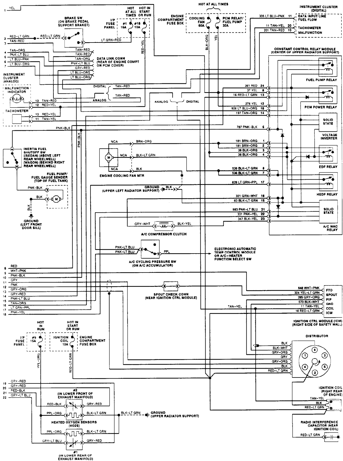
Fig. 123: EEC-IV Wiring Diagram (3.8L - 2 of 2)
