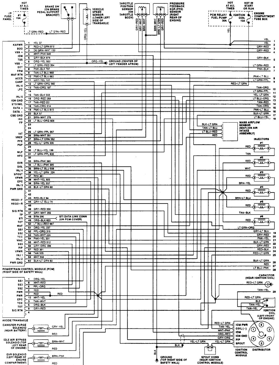
Fig. 120: EEC-IV Wiring Diagram (3.0L Except SHO 1 of 2)
