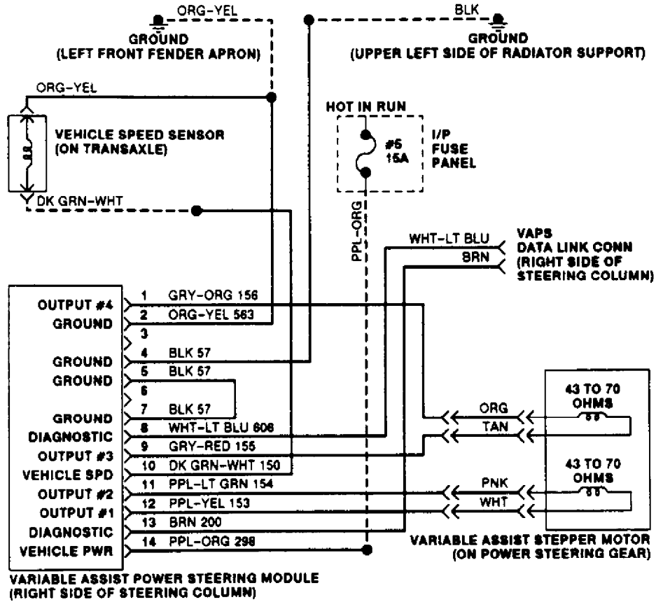
Fig. 143: Power Steering Module Wiring Diagram (SHO)
