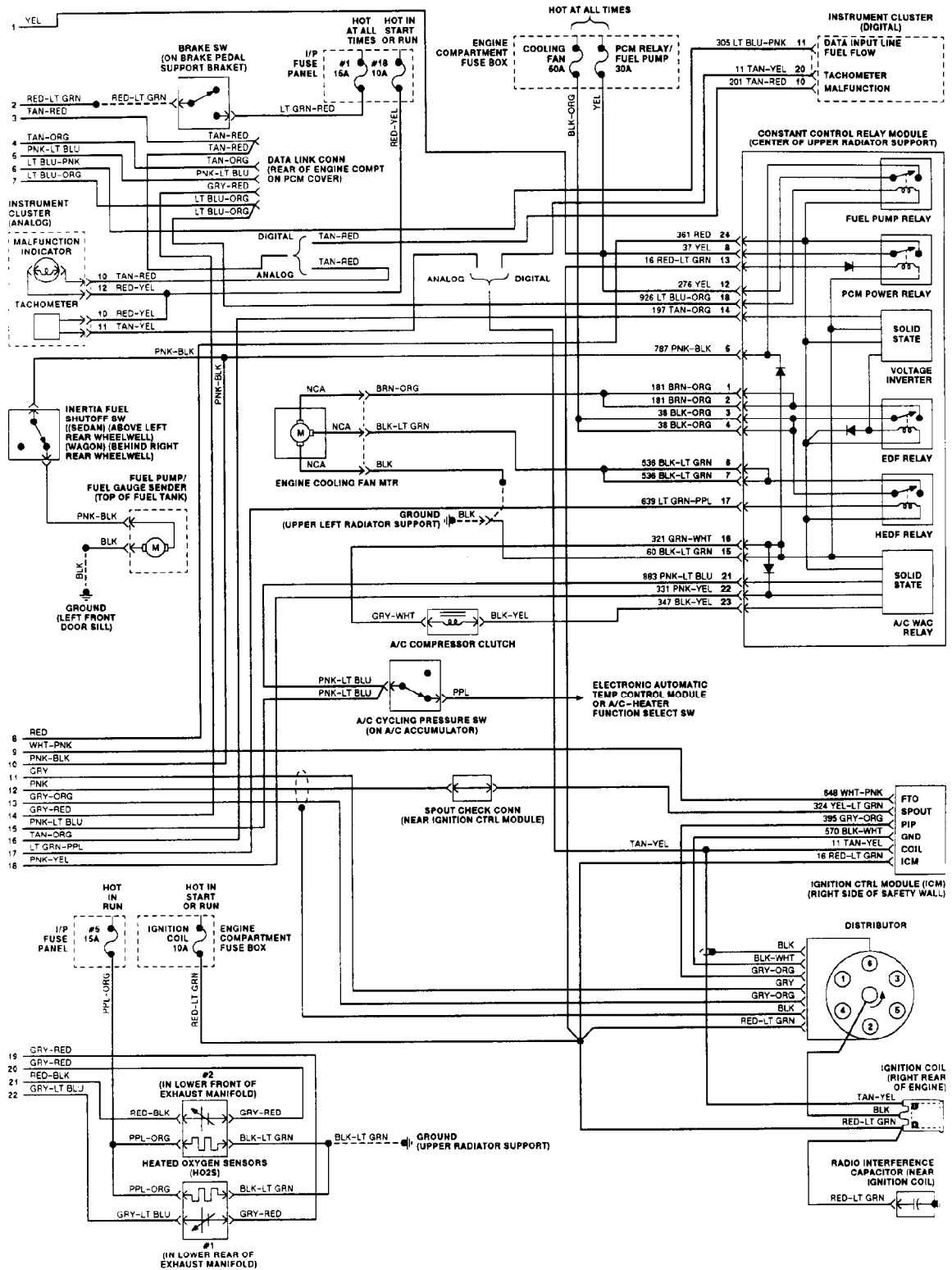
Fig. 136: EEC-IV Wiring Diagram (3.8L - 2 of 2)
