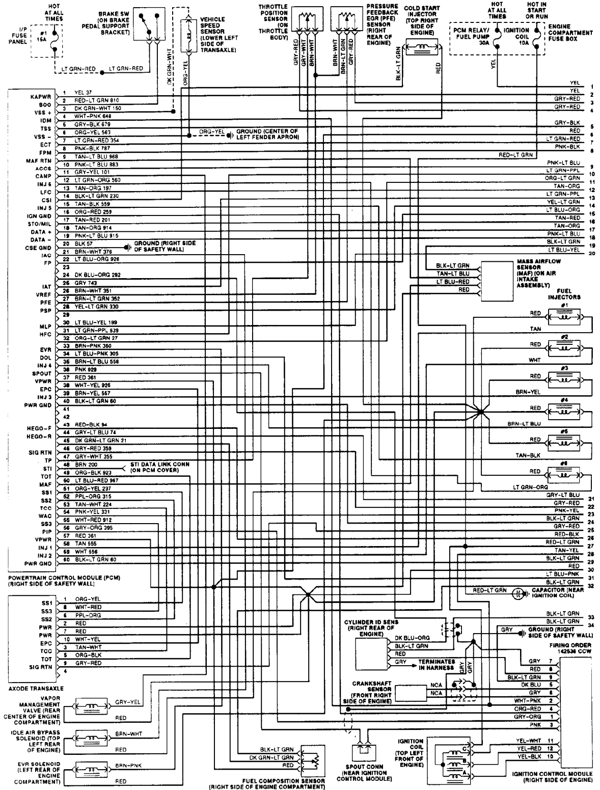
Fig. 137: EEC-IV Wiring Diagram (3.0L Flex Fuel - 1 of 2)
