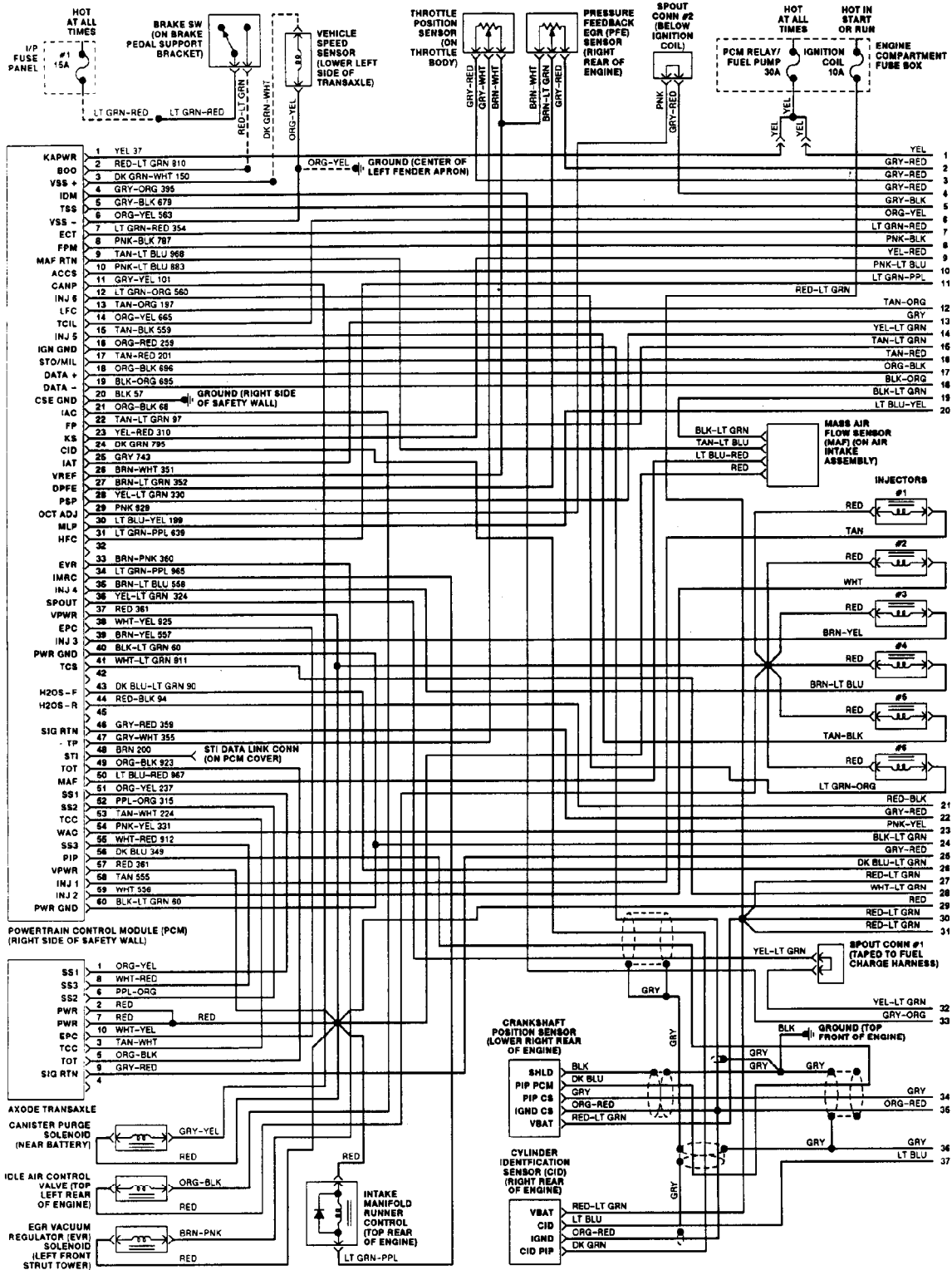
Fig. 141: EEC-IV Wiring Diagram (3.2L SHO - 1 of 2)
