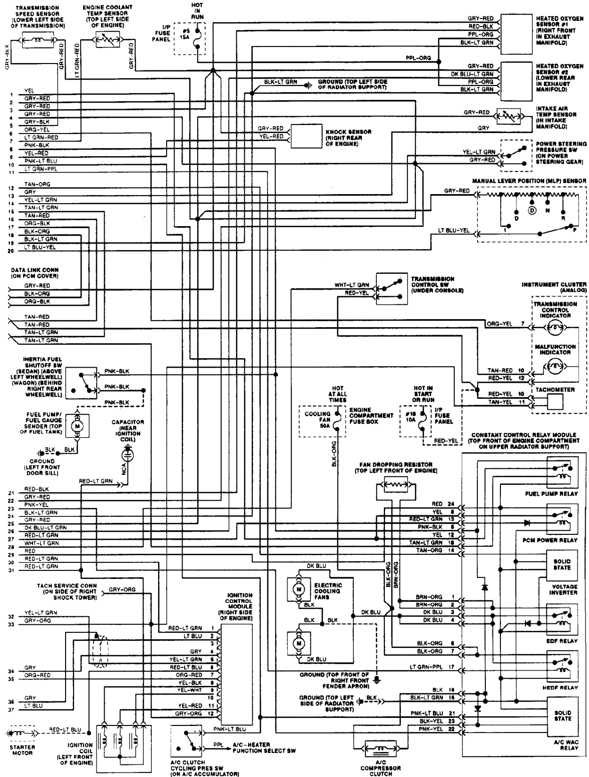
Fig. 142: EEC-IV Wiring Diagram (3.2L SHO - 2 of 2)
