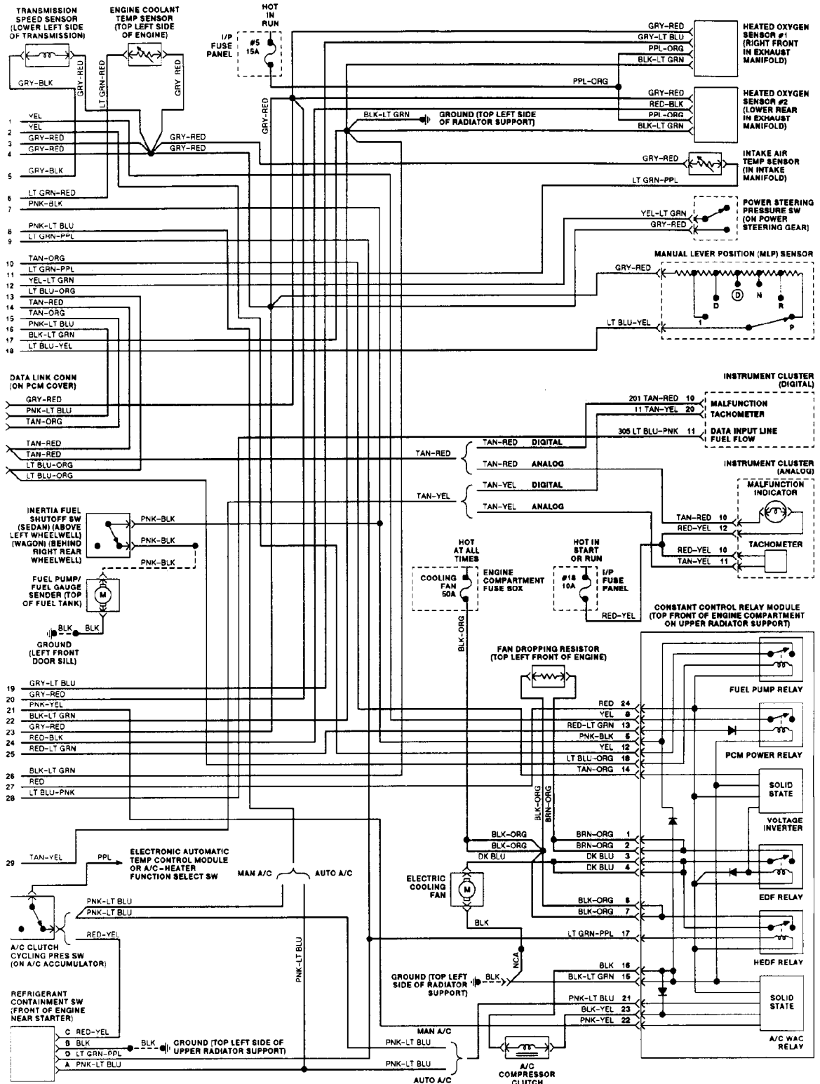
Fig. 134: EEC-IV Wiring Diagram (3.0L Except SHO 2 of 2)
