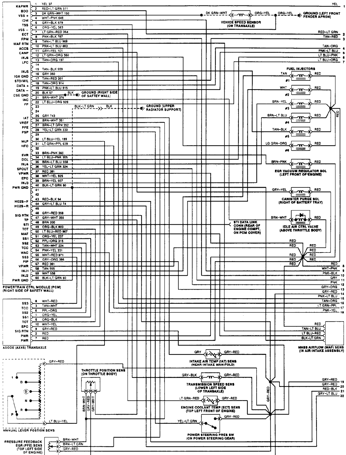
Fig. 135: EEC-IV Wiring Diagram (3.8L - 1 of 2)
