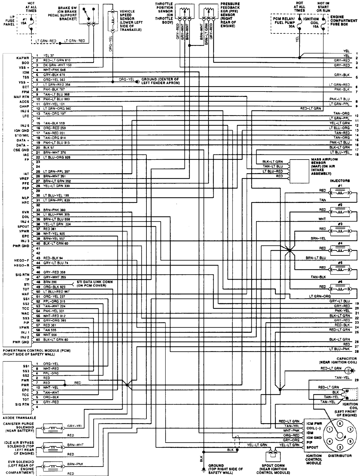
Fig. 133: EEC-IV Wiring Diagram (3.0L Except SHO 1 of 2)
