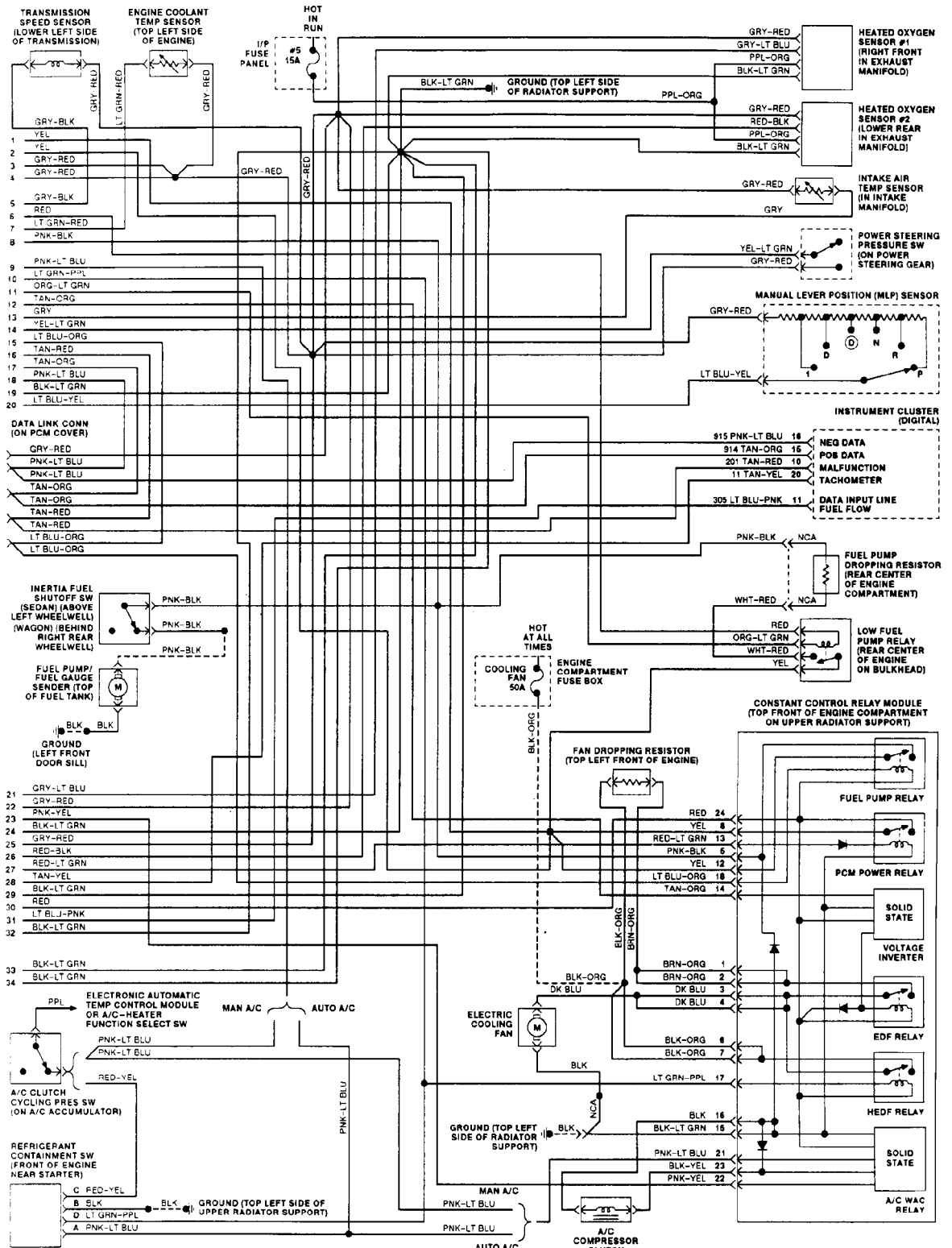
Fig. 138: EEC-IV Wiring Diagram (3.0L Flex Fuel - 2 of 2)
