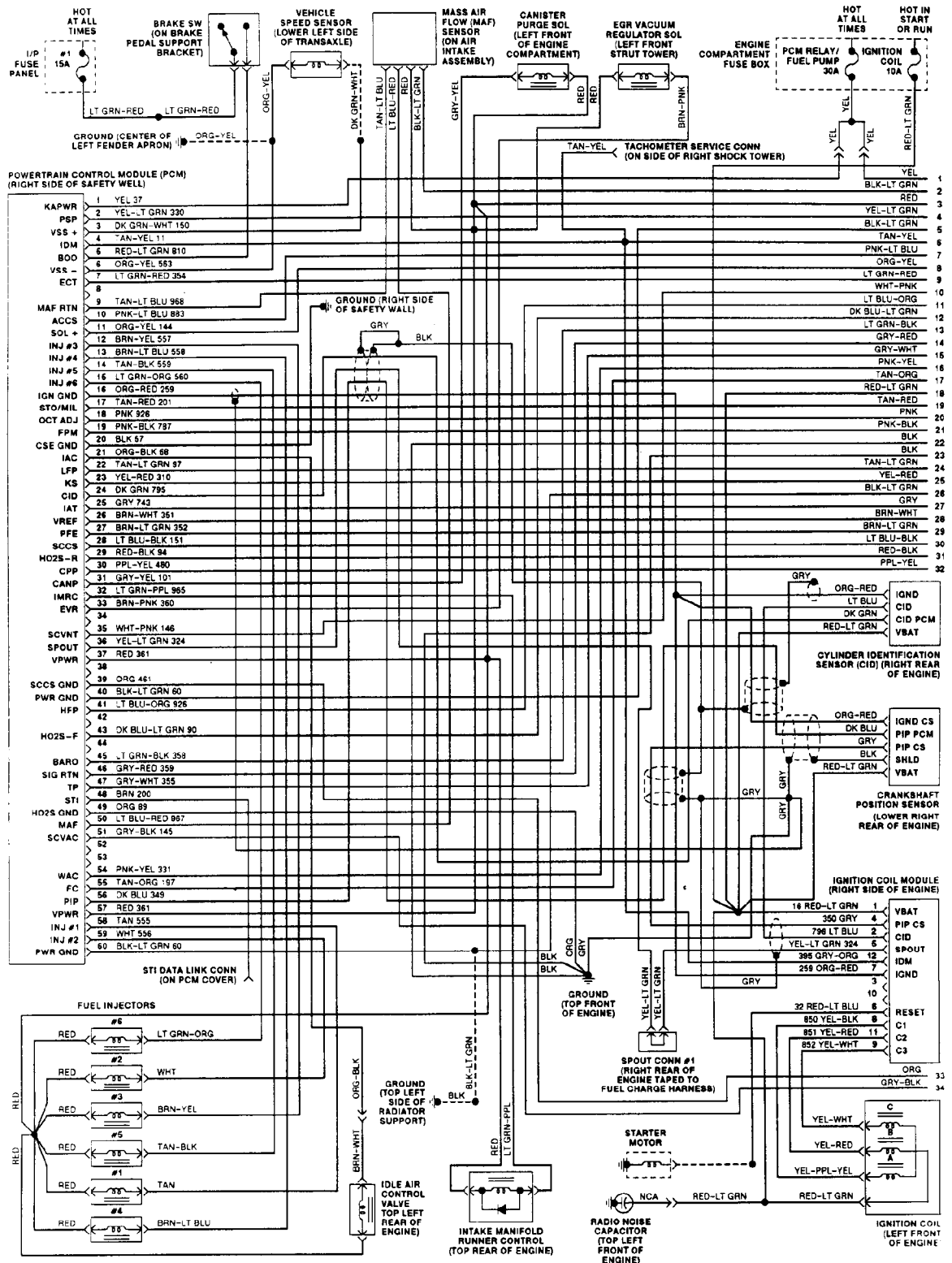
Fig. 139: EEC-IV Wiring Diagram (3.0L SHO - 1 of 2)
