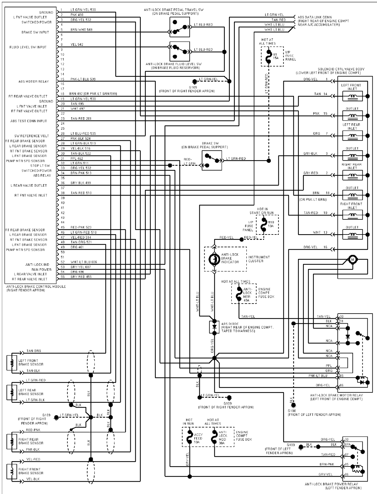
3.0L, Anti-lock Brake Circuits
