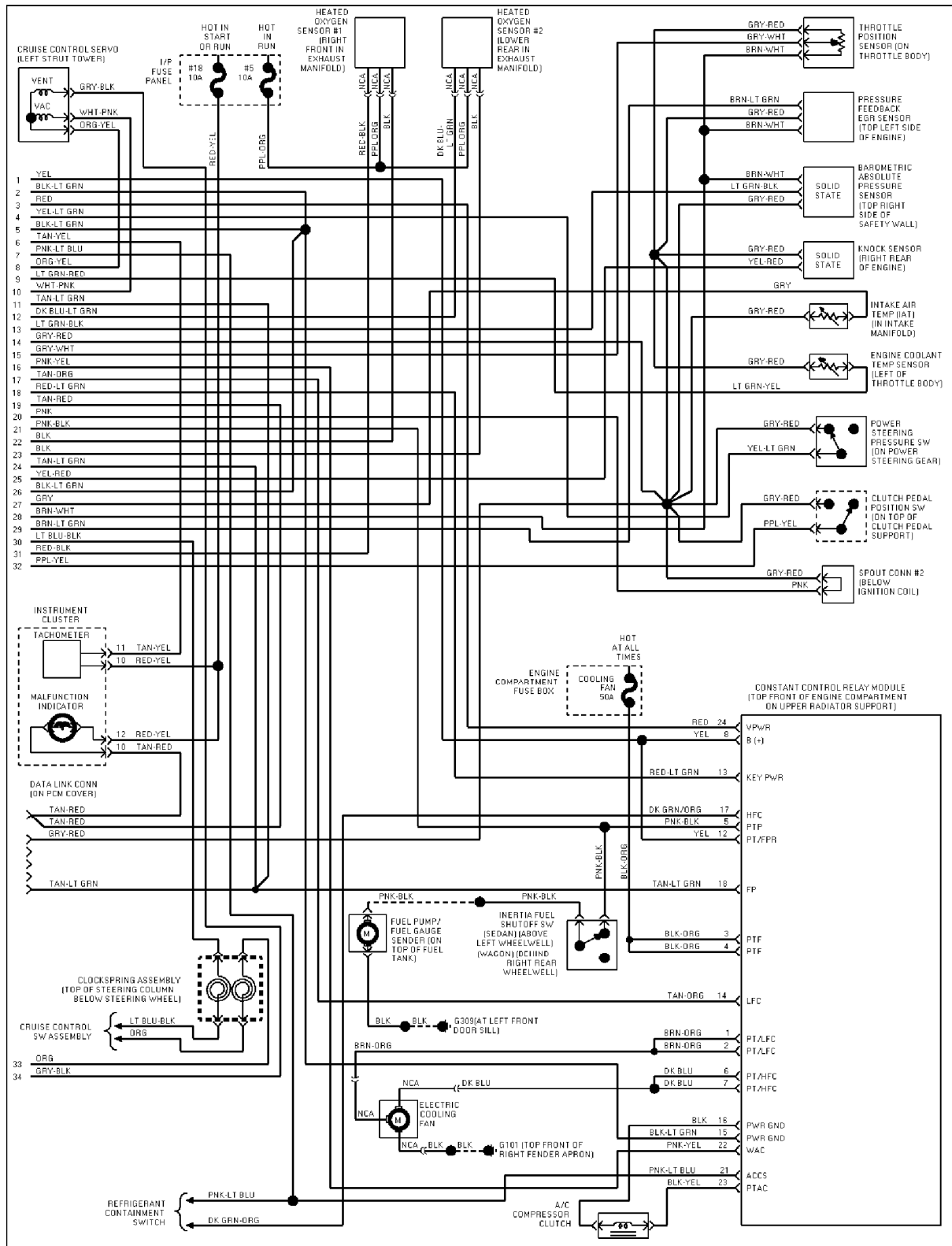
3.0L SHO, Engine Performance Circuits (2 of 2)
