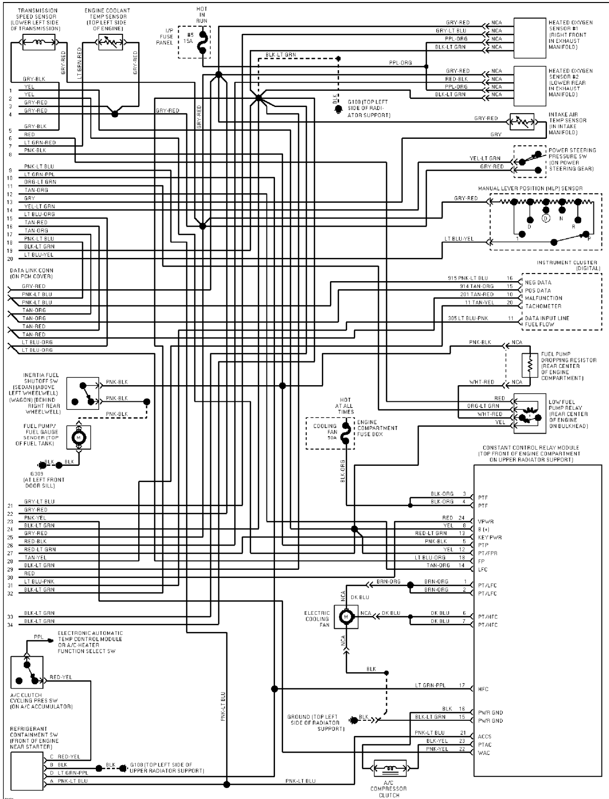
3.0L Flex Fuel, Engine Performance Circuits (2 of 2)
