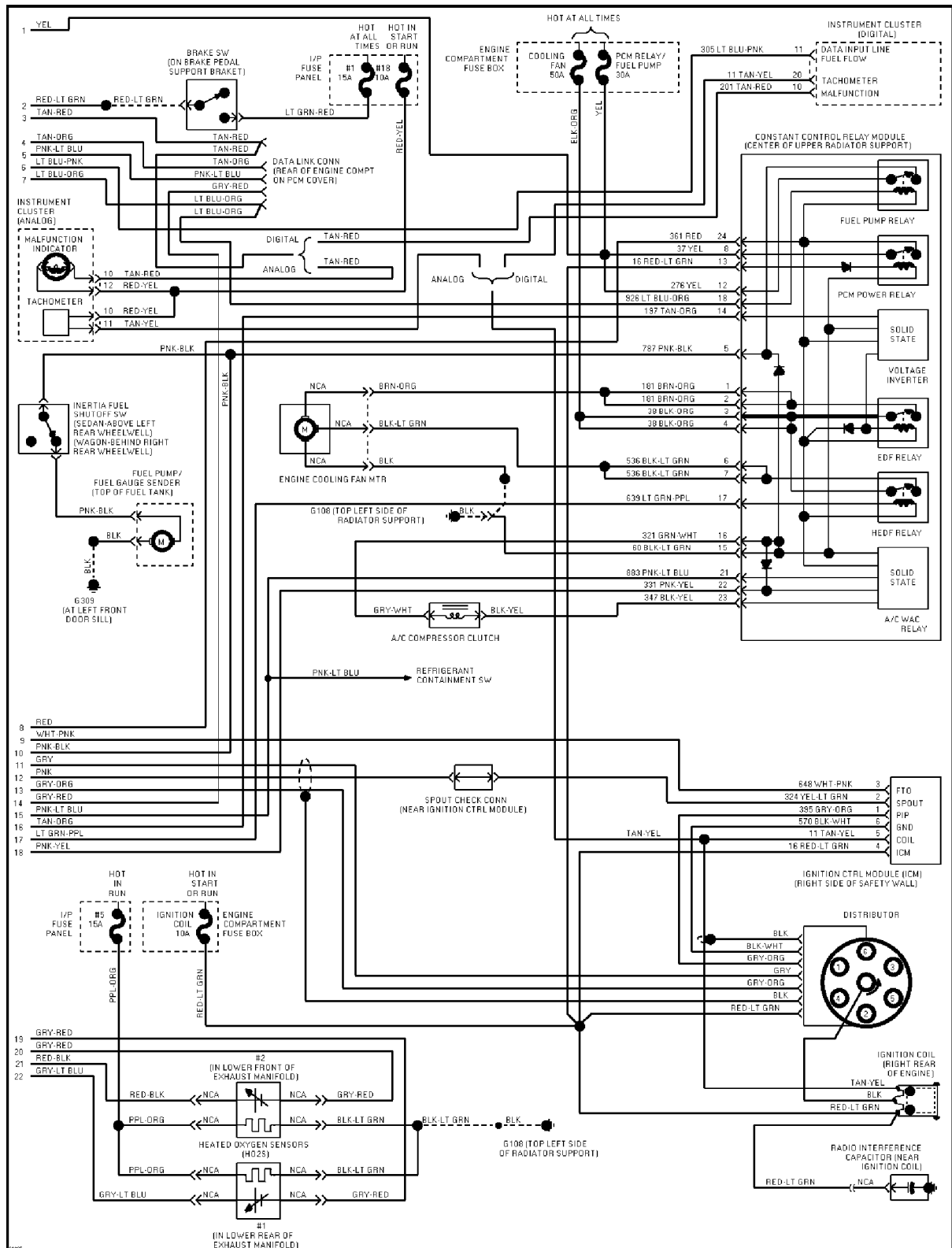
3.8L, Engine Performance Circuits (2 of 2)
