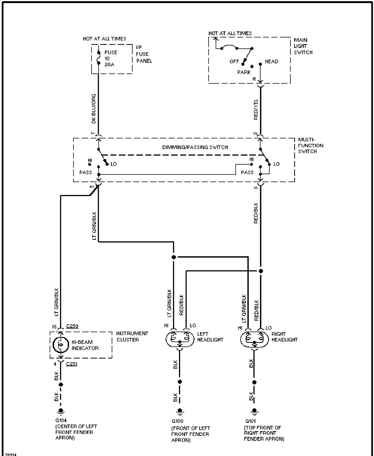
Headlamps Circuit, Base
