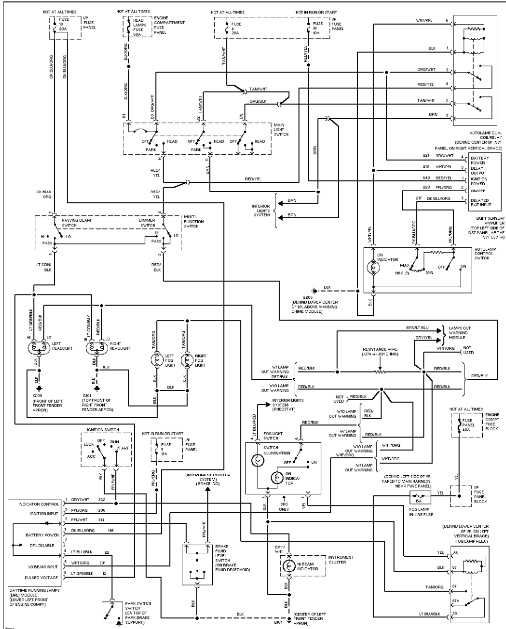
Autolamps/Fog Lamps Circuit, W/ DRL
