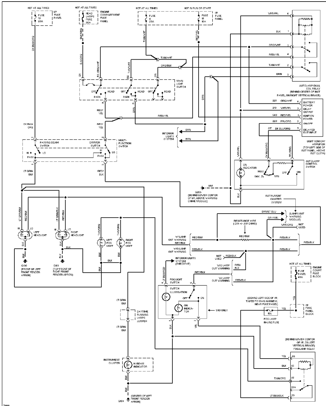
Autolamps/Fog Lamps Circuit, W/O DRL
