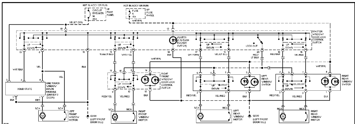
Power Window Circuit
