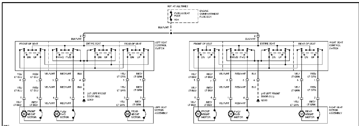
Power Seats Circuit
