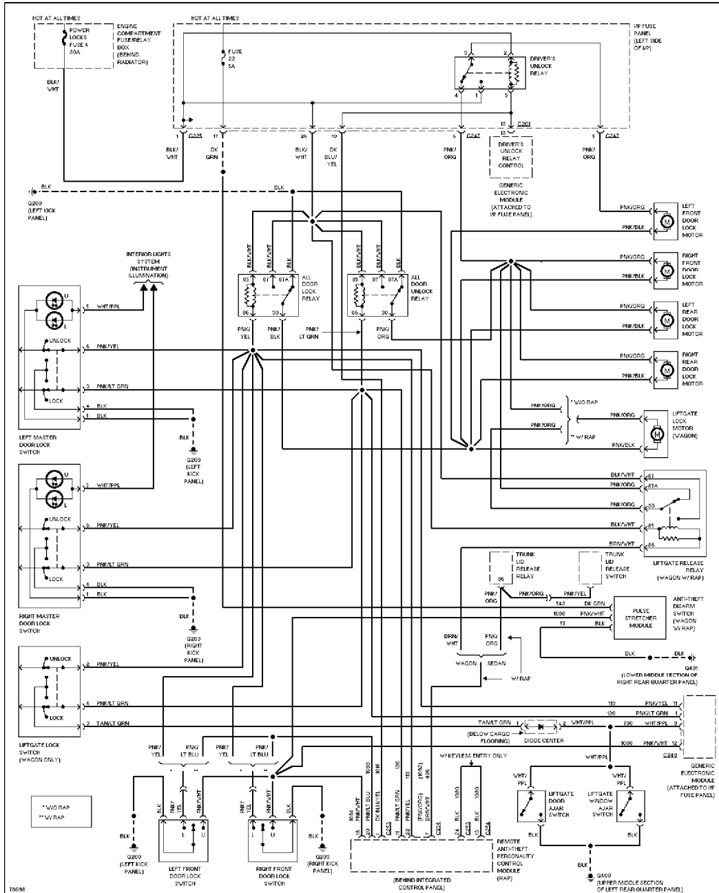
Power Door Lock Circuit
