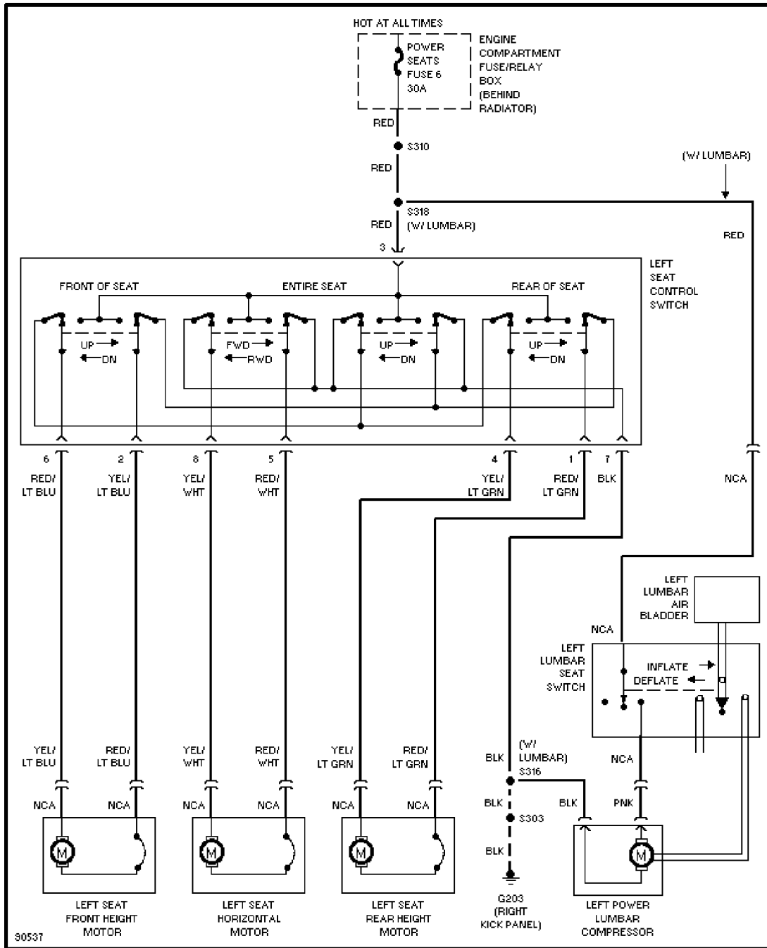
Power & Lumbar Seat Circuit
